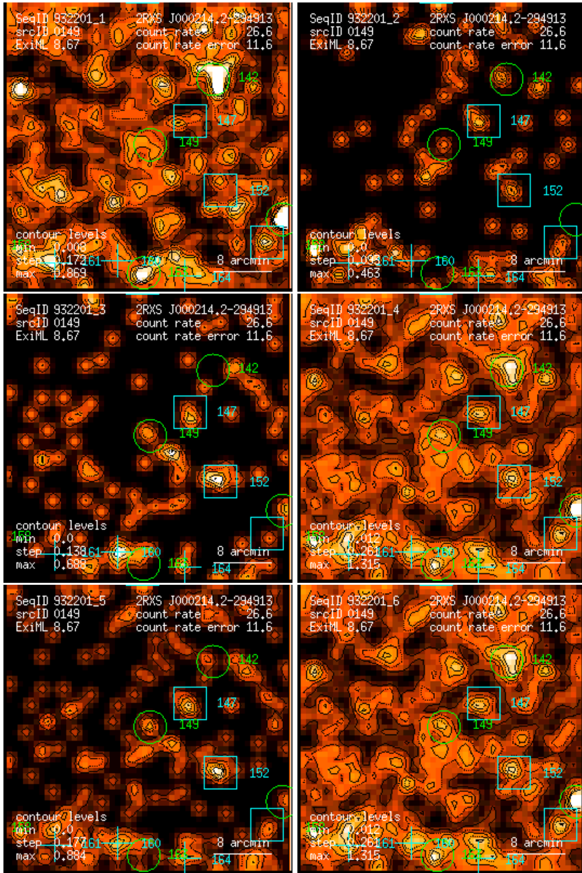
Figure 149: RASS 932201: detection 0149: band rate images, Gaussian filter: (1) PSPC channels 11 – 41, (2) 52 – 90, (3) 91 – 201, (4) 11 – 235, (5) 52 – 201, (6) 11 – 201. Broad band rates in counts/ks. Band rate contour levels in counts/ks/arcmin 2 .
