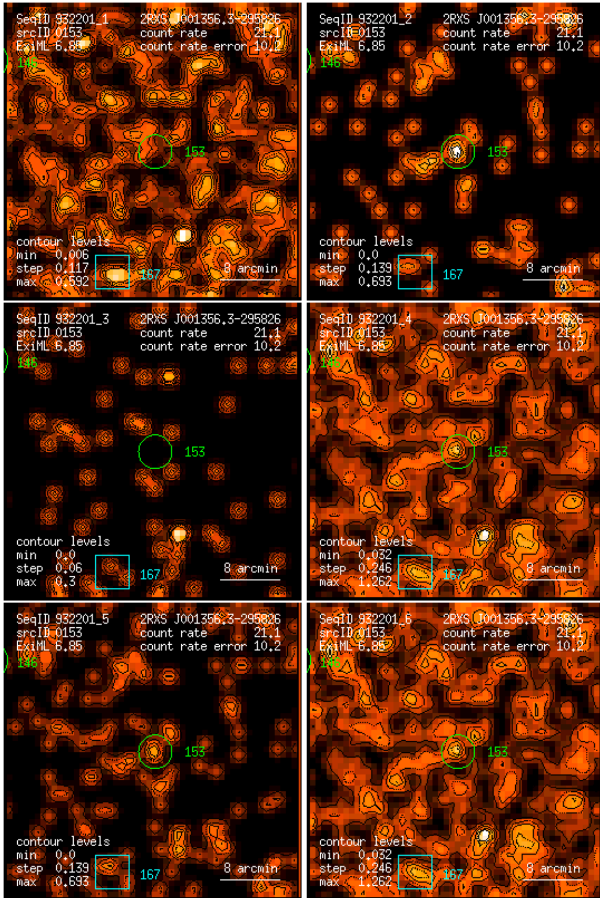
Figure 153: RASS 932201: detection 0153: band rate images, Gaussian filter: (1) PSPC channels 11 – 41, (2) 52 – 90, (3) 91 – 201, (4) 11 – 235, (5) 52 – 201, (6) 11 – 201. Broad band rates in counts/ks. Band rate contour levels in counts/ks/arcmin 2 .
