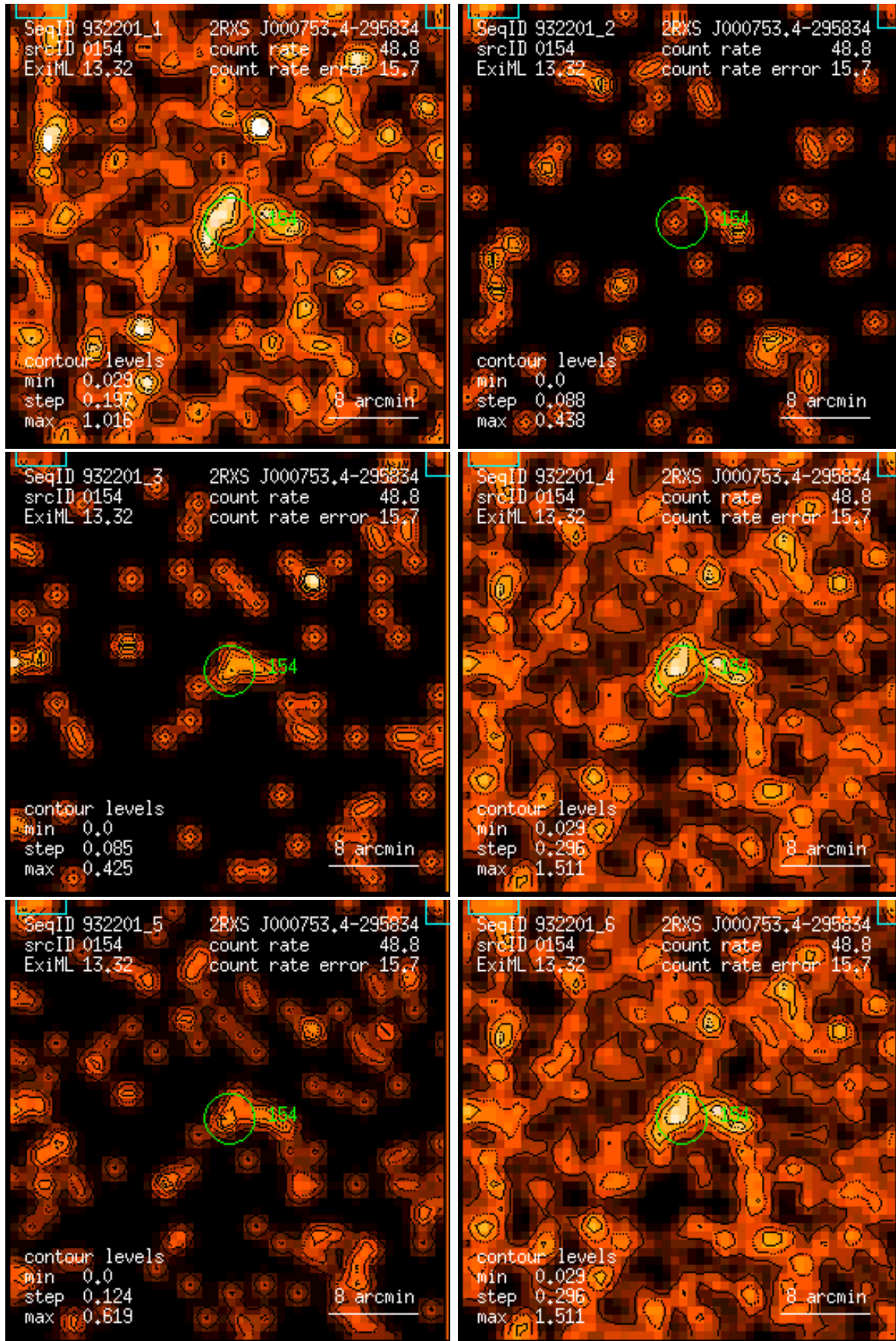
Figure 154: RASS 932201: detection 0154: band rate images, Gaussian filter: (1) PSPC channels 11 – 41, (2) 52 – 90, (3) 91 – 201, (4) 11 – 235, (5) 52 – 201, (6) 11 – 201. Broad band rates in counts/ks. Band rate contour levels in counts/ks/arcmin 2 .
