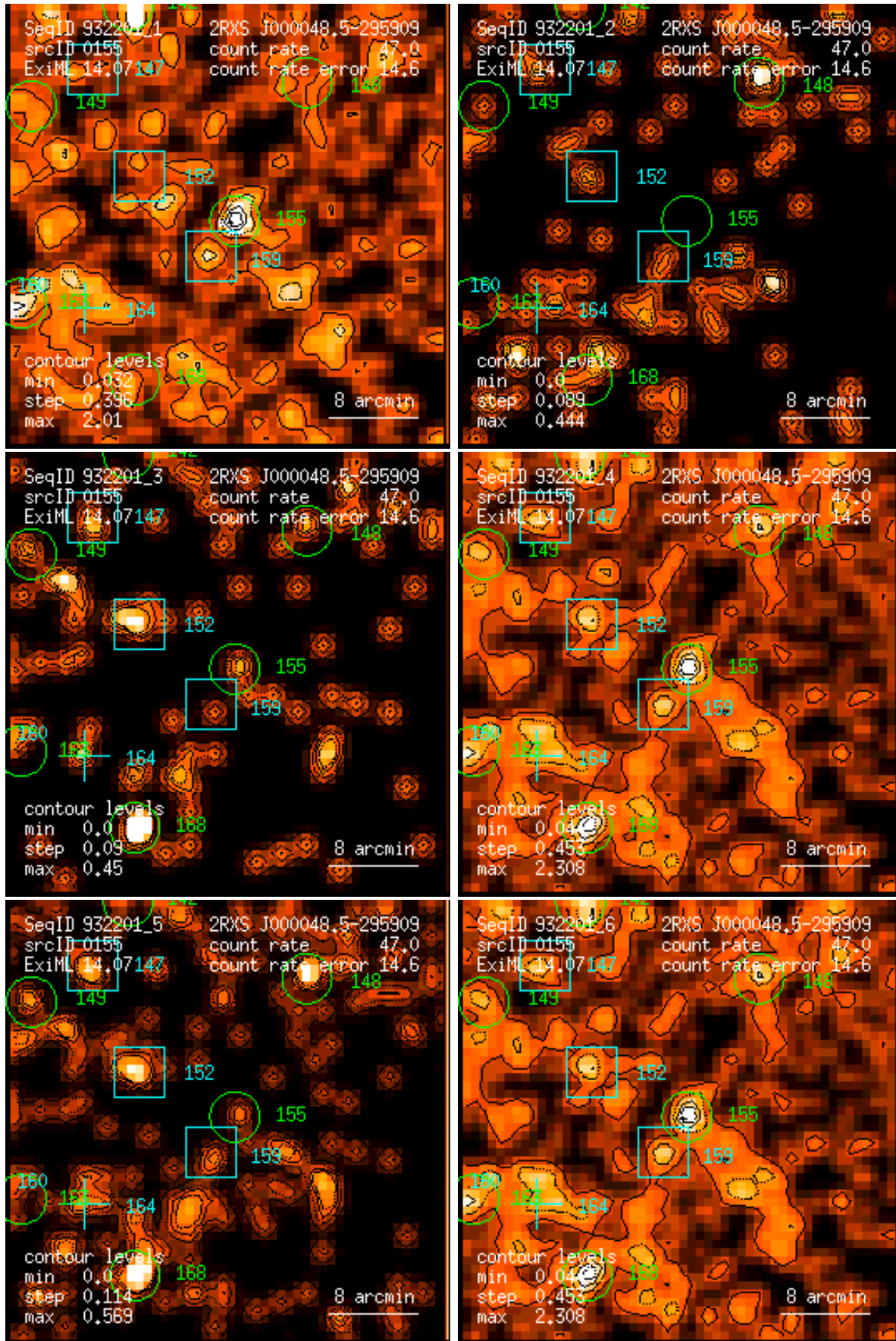
Figure 155: RASS 932201: detection 0155: band rate images, Gaussian filter: (1) PSPC channels 11 – 41, (2) 52 – 90, (3) 91 – 201, (4) 11 – 235, (5) 52 – 201, (6) 11 – 201. Broad band rates in counts/ks. Band rate contour levels in counts/ks/arcmin 2 .
