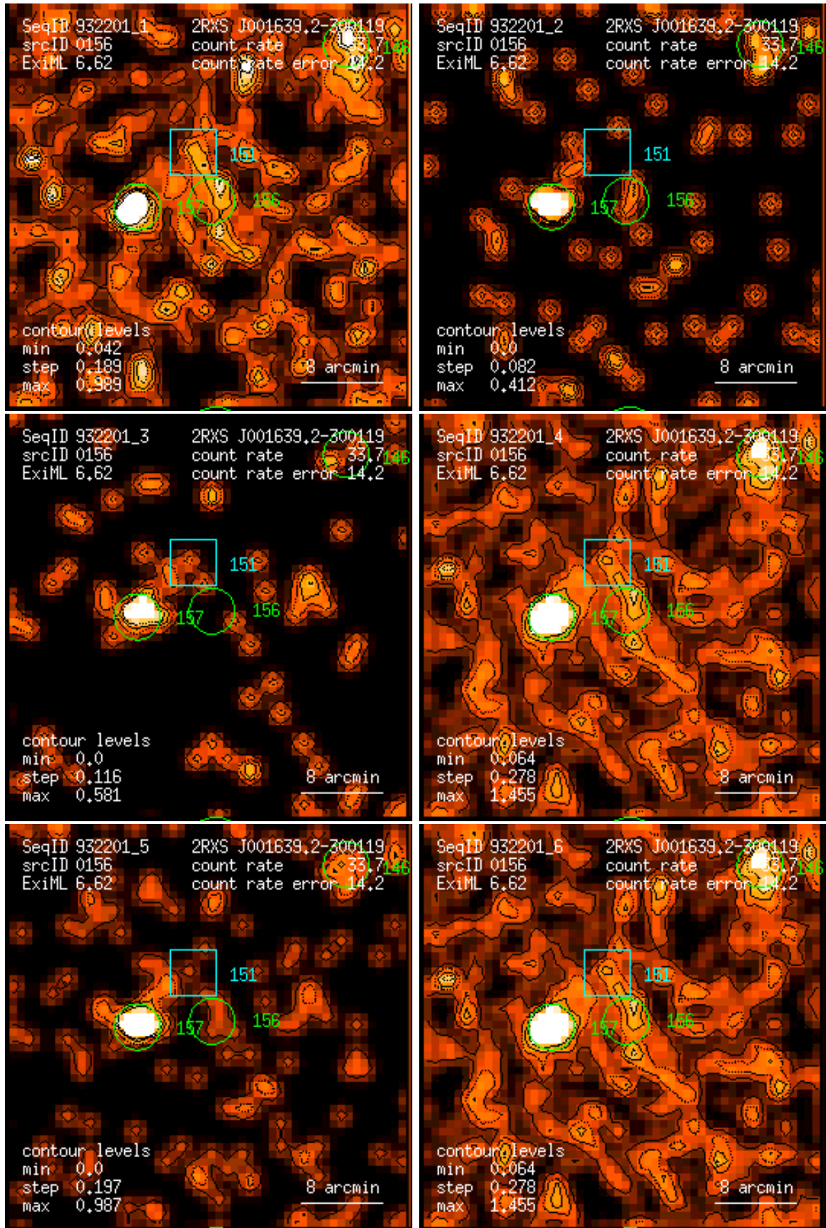
Figure 156: RASS 932201: detection 0156: band rate images, Gaussian filter: (1) PSPC channels 11 – 41, (2) 52 – 90, (3) 91 – 201, (4) 11 – 235, (5) 52 – 201, (6) 11 – 201. Broad band rates in counts/ks. Band rate contour levels in counts/ks/arcmin 2 .
