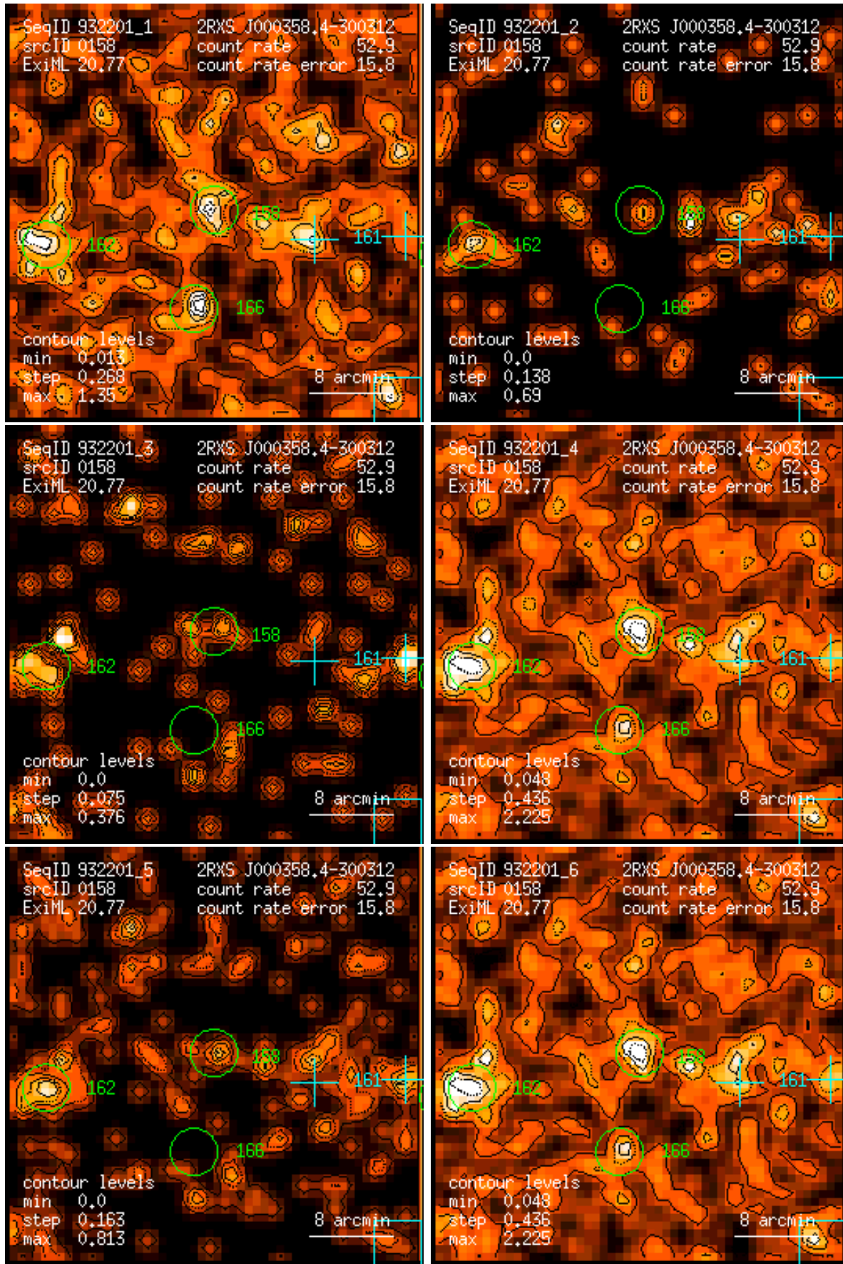
Figure 158: RASS 932201: detection 0158: band rate images, Gaussian filter: (1) PSPC channels 11 – 41, (2) 52 – 90, (3) 91 – 201, (4) 11 – 235, (5) 52 – 201, (6) 11 – 201. Broad band rates in counts/ks. Band rate contour levels in counts/ks/arcmin 2 .
