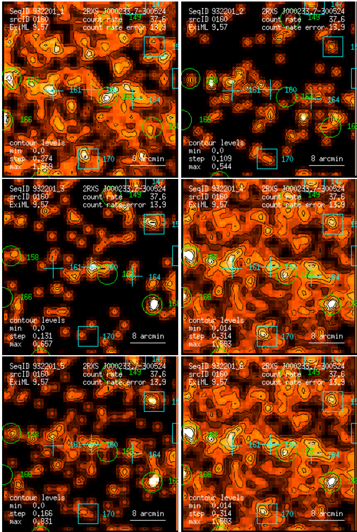
Figure 160: RASS 932201: detection 0160: band rate images, Gaussian filter: (1) PSPC channels 11 – 41, (2) 52 – 90, (3) 91 – 201, (4) 11 – 235, (5) 52 – 201, (6) 11 – 201. Broad band rates in counts/ks. Band rate contour levels in counts/ks/arcmin 2 .
