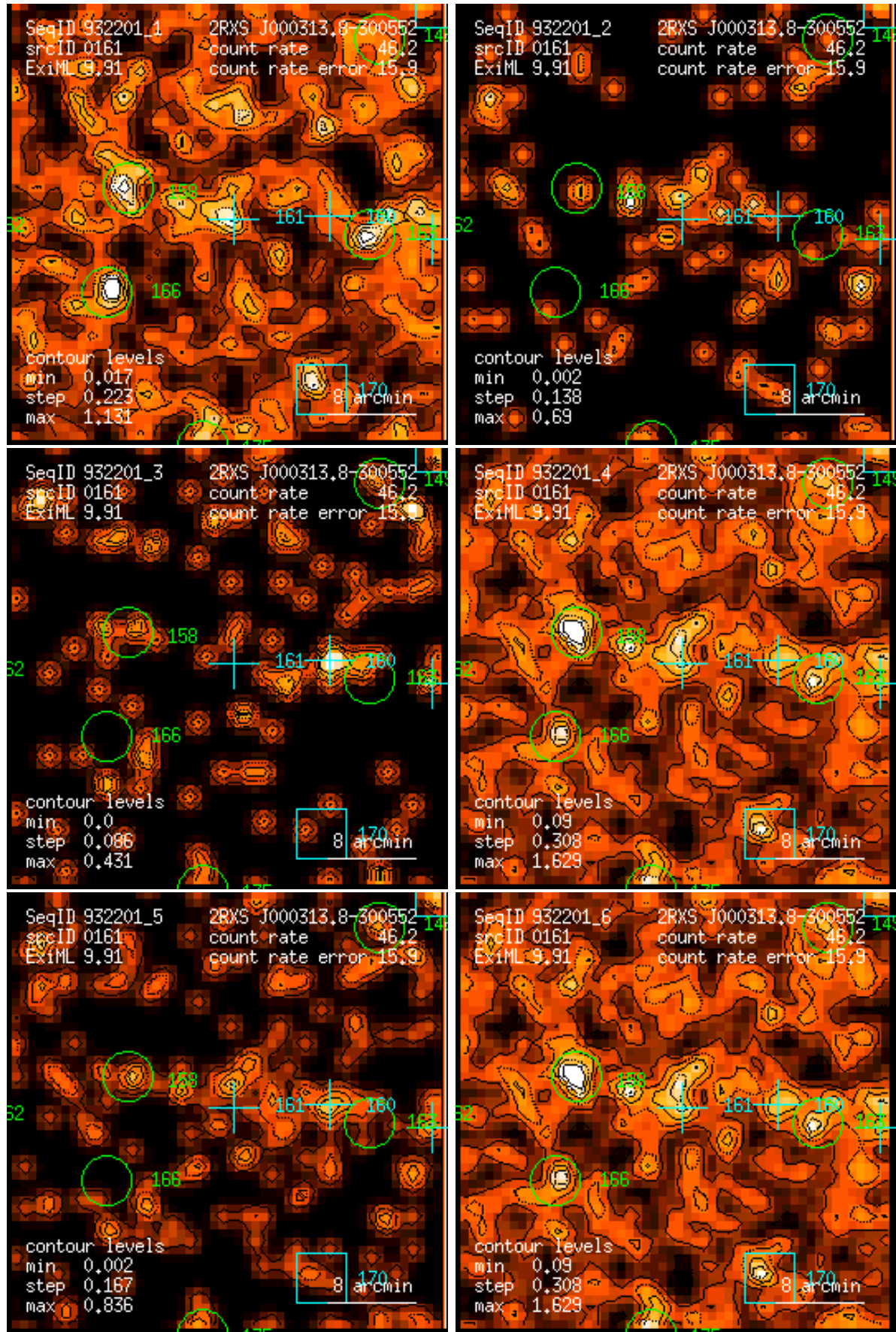
Figure 161: RASS 932201: detection 0161: band rate images, Gaussian filter: (1) PSPC channels 11 – 41, (2) 52 – 90, (3) 91 – 201, (4) 11 – 235, (5) 52 – 201, (6) 11 – 201. Broad band rates in counts/ks. Band rate contour levels in counts/ks/arcmin 2 .
