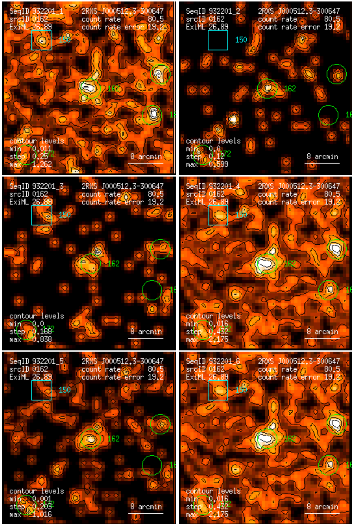
Figure 162: RASS 932201: detection 0162: band rate images, Gaussian filter: (1) PSPC channels 11 – 41, (2) 52 – 90, (3) 91 – 201, (4) 11 – 235, (5) 52 – 201, (6) 11 – 201. Broad band rates in counts/ks. Band rate contour levels in counts/ks/arcmin 2 .
