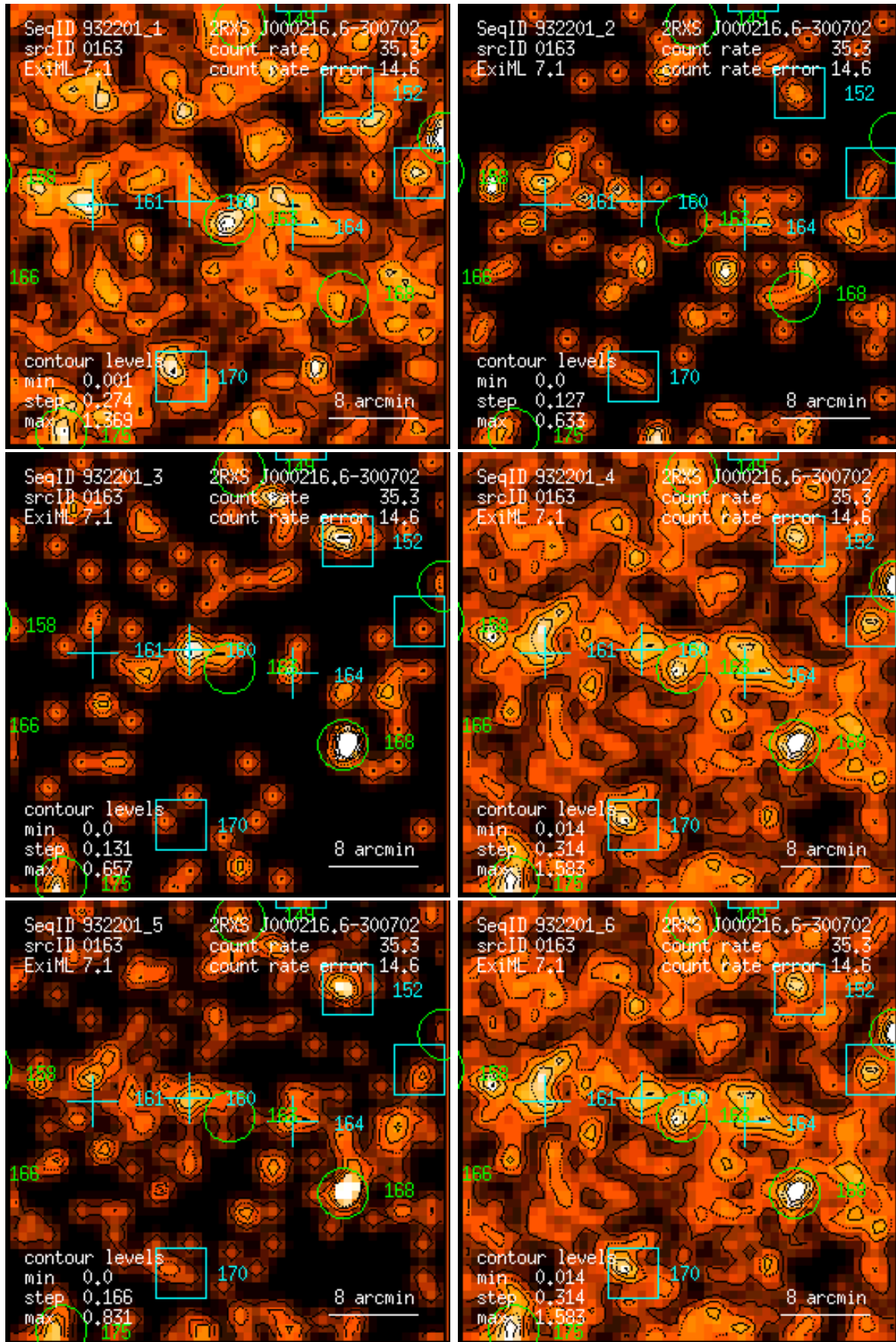
Figure 163: RASS 932201: detection 0163: band rate images, Gaussian filter: (1) PSPC channels 11 – 41, (2) 52 – 90, (3) 91 – 201, (4) 11 – 235, (5) 52 – 201, (6) 11 – 201. Broad band rates in counts/ks. Band rate contour levels in counts/ks/arcmin 2 .
