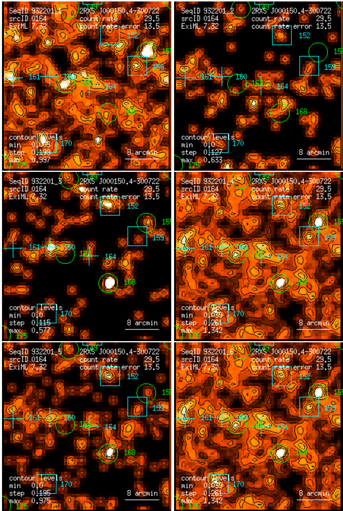
Figure 164: RASS 932201: detection 0164: band rate images, Gaussian filter: (1) PSPC channels 11 – 41, (2) 52 – 90, (3) 91 – 201, (4) 11 – 235, (5) 52 – 201, (6) 11 – 201. Broad band rates in counts/ks. Band rate contour levels in counts/ks/arcmin 2 .
