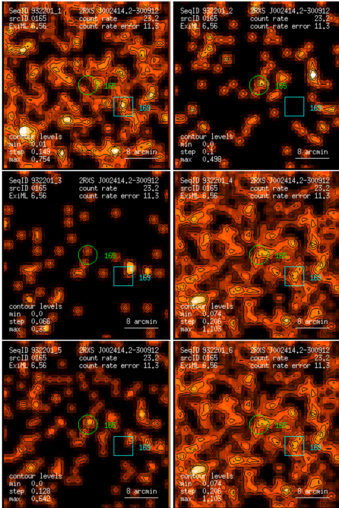
Figure 165: RASS 932201: detection 0165: band rate images, Gaussian filter: (1) PSPC channels 11 – 41, (2) 52 – 90, (3) 91 – 201, (4) 11 – 235, (5) 52 – 201, (6) 11 – 201. Broad band rates in counts/ks. Band rate contour levels in counts/ks/arcmin 2 .
