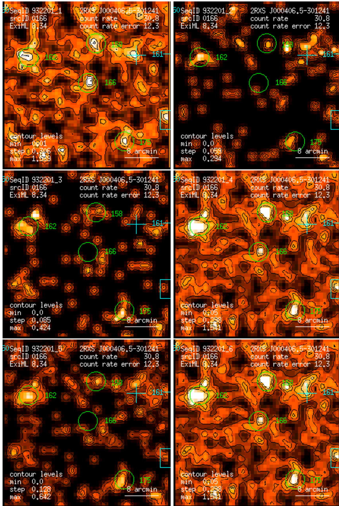
Figure 166: RASS 932201: detection 0166: band rate images, Gaussian filter: (1) PSPC channels 11 – 41, (2) 52 – 90, (3) 91 – 201, (4) 11 – 235, (5) 52 – 201, (6) 11 – 201. Broad band rates in counts/ks. Band rate contour levels in counts/ks/arcmin 2 .
