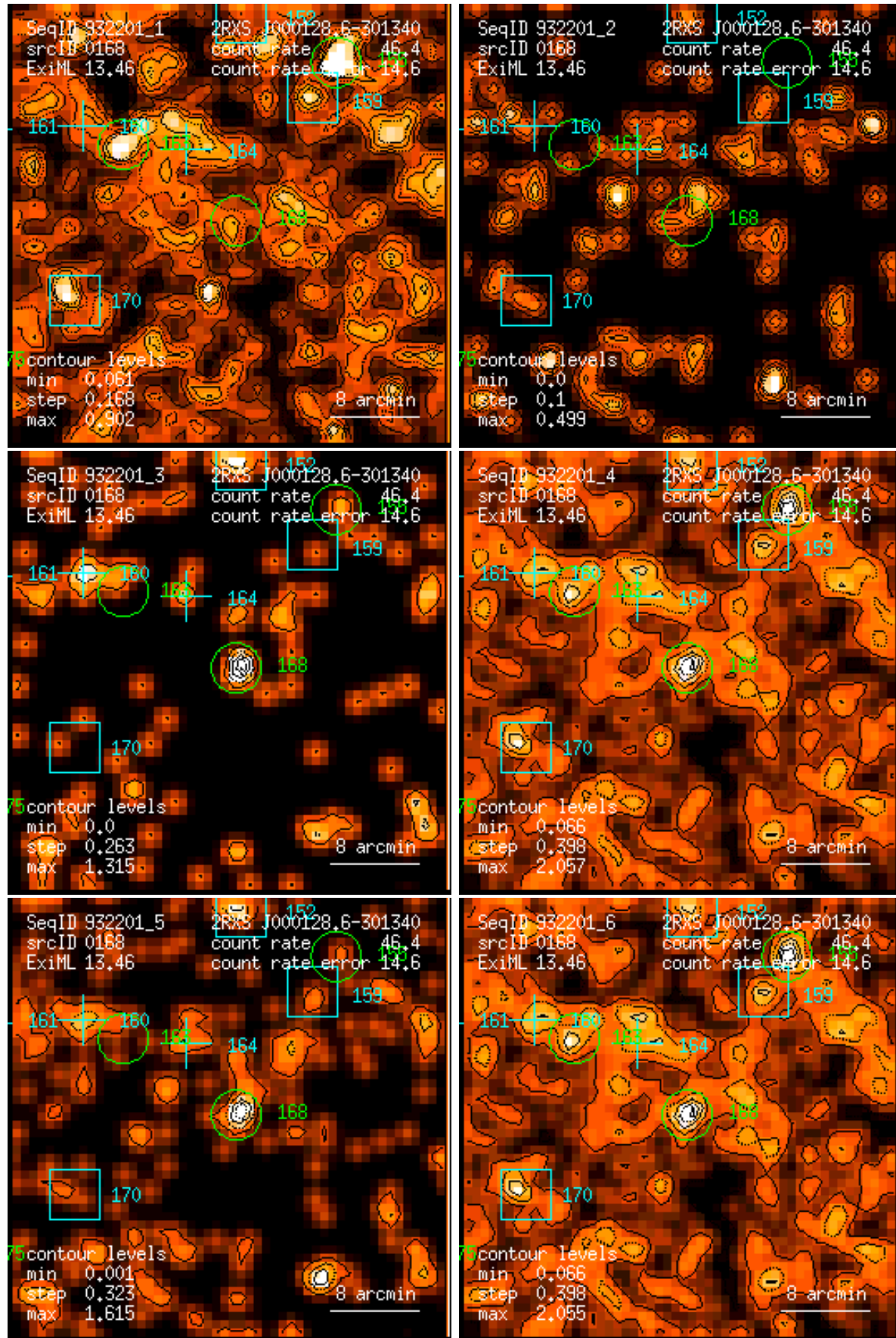
Figure 168: RASS 932201: detection 0168: band rate images, Gaussian filter: (1) PSPC channels 11 – 41, (2) 52 – 90, (3) 91 – 201, (4) 11 – 235, (5) 52 – 201, (6) 11 – 201. Broad band rates in counts/ks. Band rate contour levels in counts/ks/arcmin 2 .
