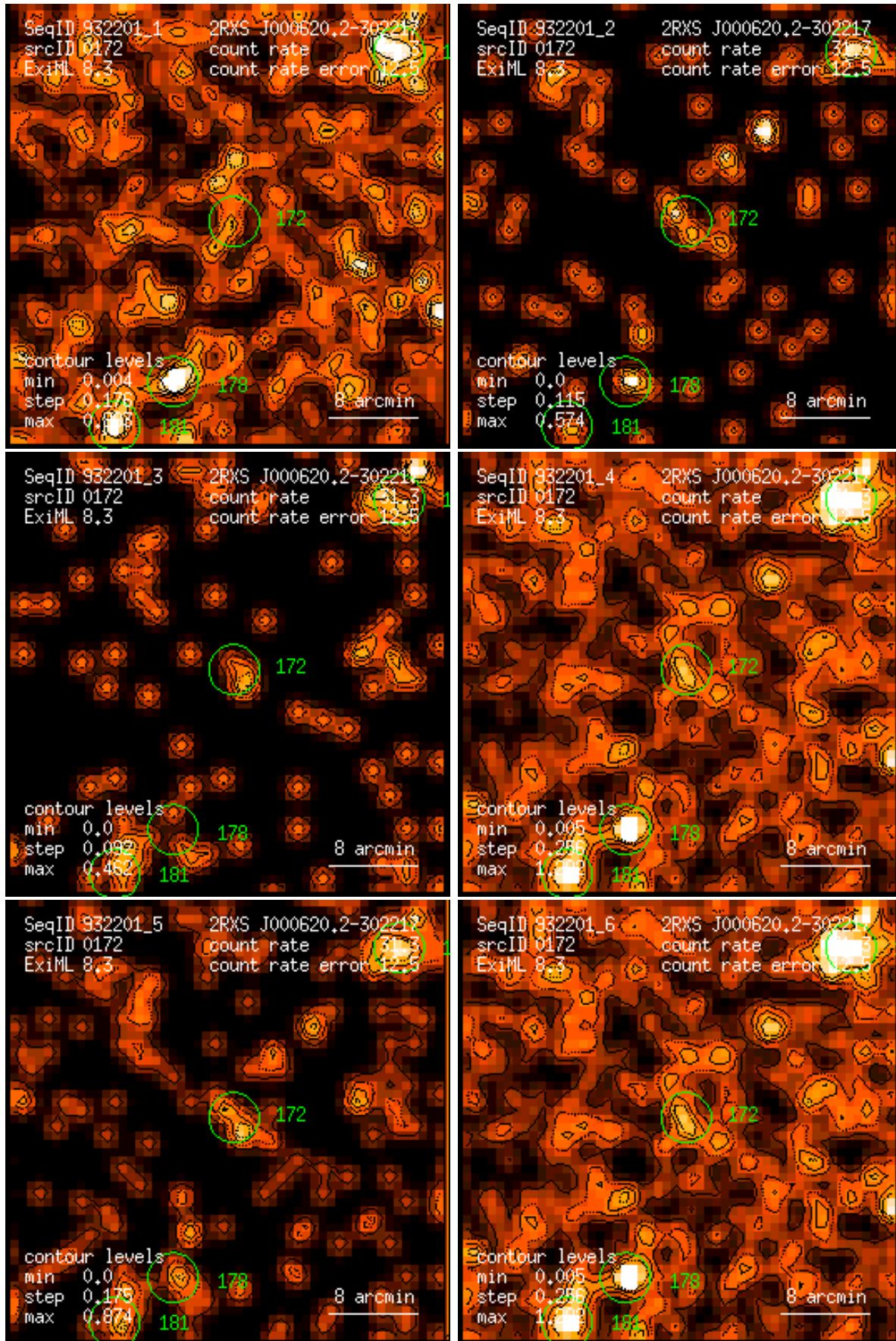
Figure 172: RASS 932201: detection 0172: band rate images, Gaussian filter: (1) PSPC channels 11 – 41, (2) 52 – 90, (3) 91 – 201, (4) 11 – 235, (5) 52 – 201, (6) 11 – 201. Broad band rates in counts/ks. Band rate contour levels in counts/ks/arcmin 2 .
