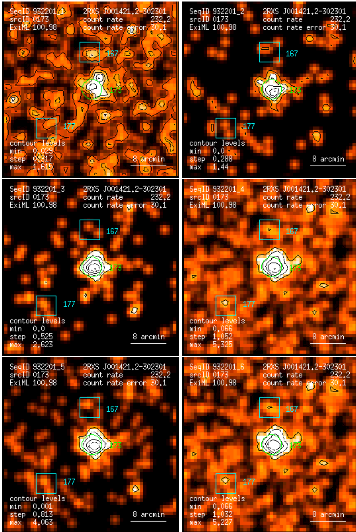
Figure 173: RASS 932201: detection 0173: band rate images, Gaussian filter: (1) PSPC channels 11 – 41, (2) 52 – 90, (3) 91 – 201, (4) 11 – 235, (5) 52 – 201, (6) 11 – 201. Broad band rates in counts/ks. Band rate contour levels in counts/ks/arcmin 2 .
