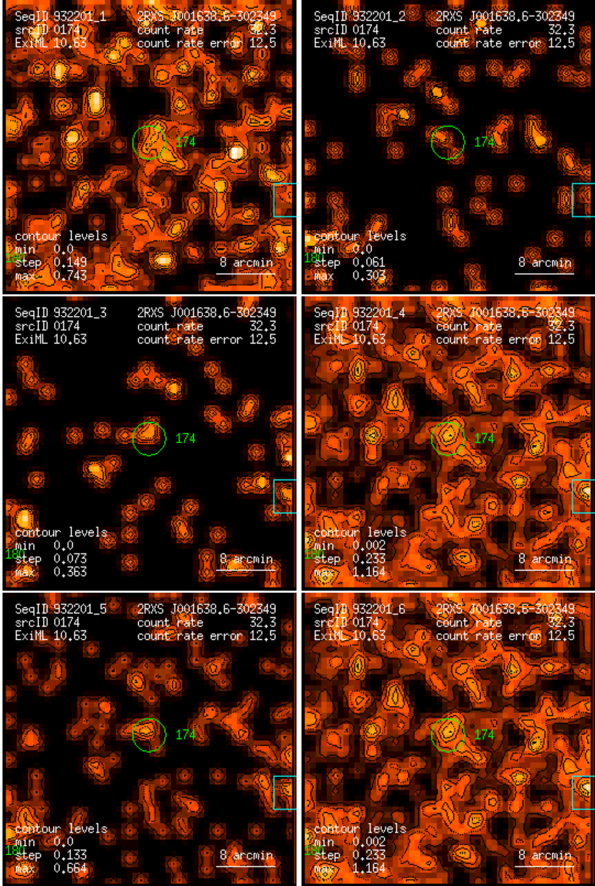
Figure 174: RASS 932201: detection 0174: band rate images, Gaussian filter: (1) PSPC channels 11 – 41, (2) 52 – 90, (3) 91 – 201, (4) 11 – 235, (5) 52 – 201, (6) 11 – 201. Broad band rates in counts/ks. Band rate contour levels in counts/ks/arcmin 2 .
