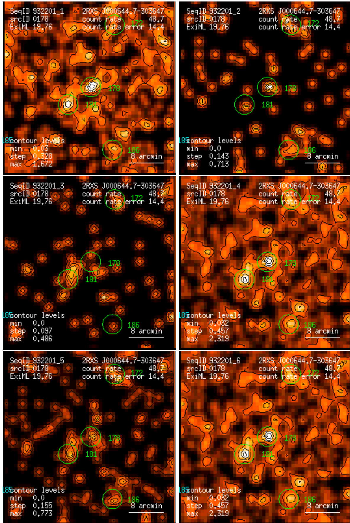
Figure 178: RASS 932201: detection 0178: band rate images, Gaussian filter: (1) PSPC channels 11 – 41, (2) 52 – 90, (3) 91 – 201, (4) 11 – 235, (5) 52 – 201, (6) 11 – 201. Broad band rates in counts/ks. Band rate contour levels in counts/ks/arcmin 2 .
