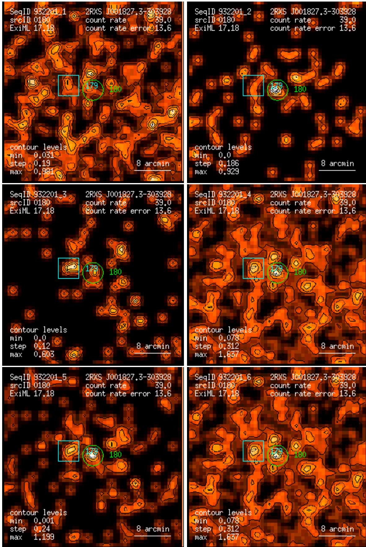
Figure 180: RASS 932201: detection 0180: band rate images, Gaussian filter: (1) PSPC channels 11 – 41, (2) 52 – 90, (3) 91 – 201, (4) 11 – 235, (5) 52 – 201, (6) 11 – 201. Broad band rates in counts/ks. Band rate contour levels in counts/ks/arcmin 2 .
