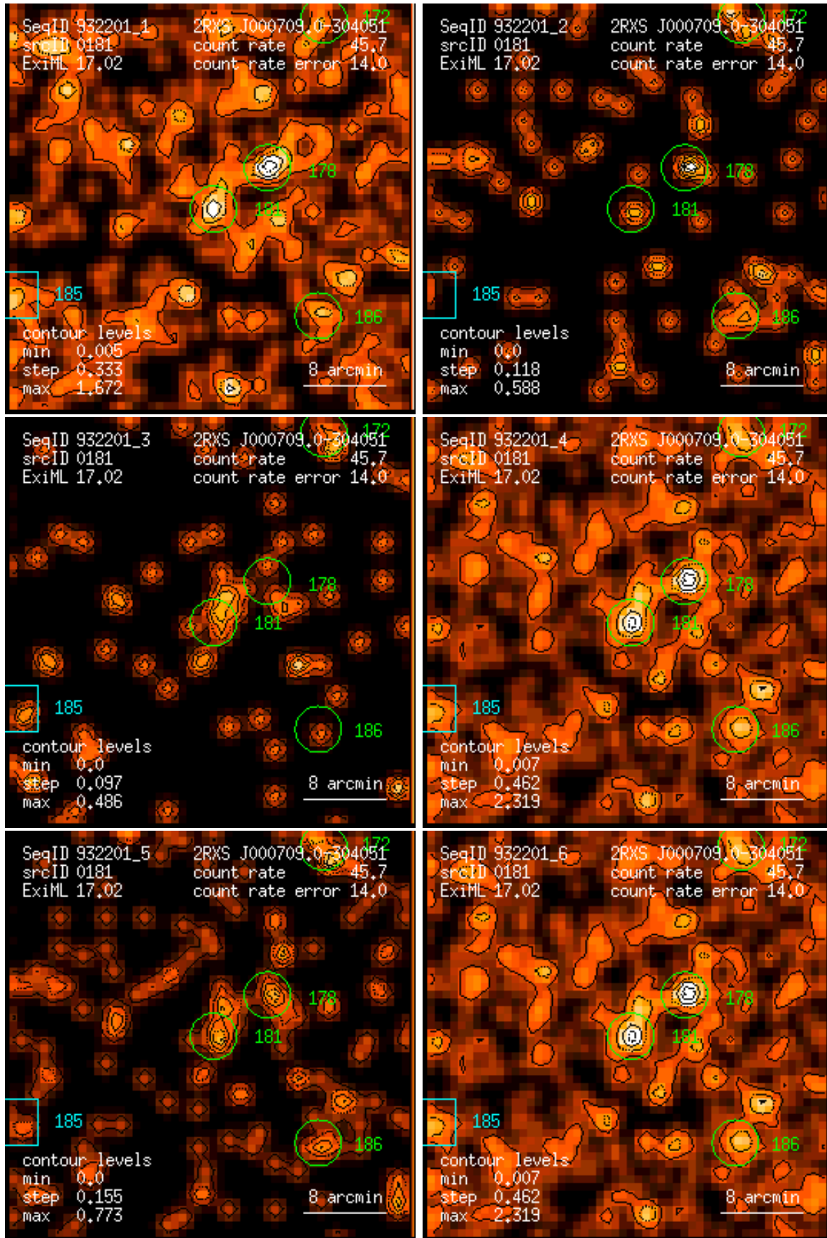
Figure 181: RASS 932201: detection 0181: band rate images, Gaussian filter: (1) PSPC channels 11 – 41, (2) 52 – 90, (3) 91 – 201, (4) 11 – 235, (5) 52 – 201, (6) 11 – 201. Broad band rates in counts/ks. Band rate contour levels in counts/ks/arcmin 2 .
