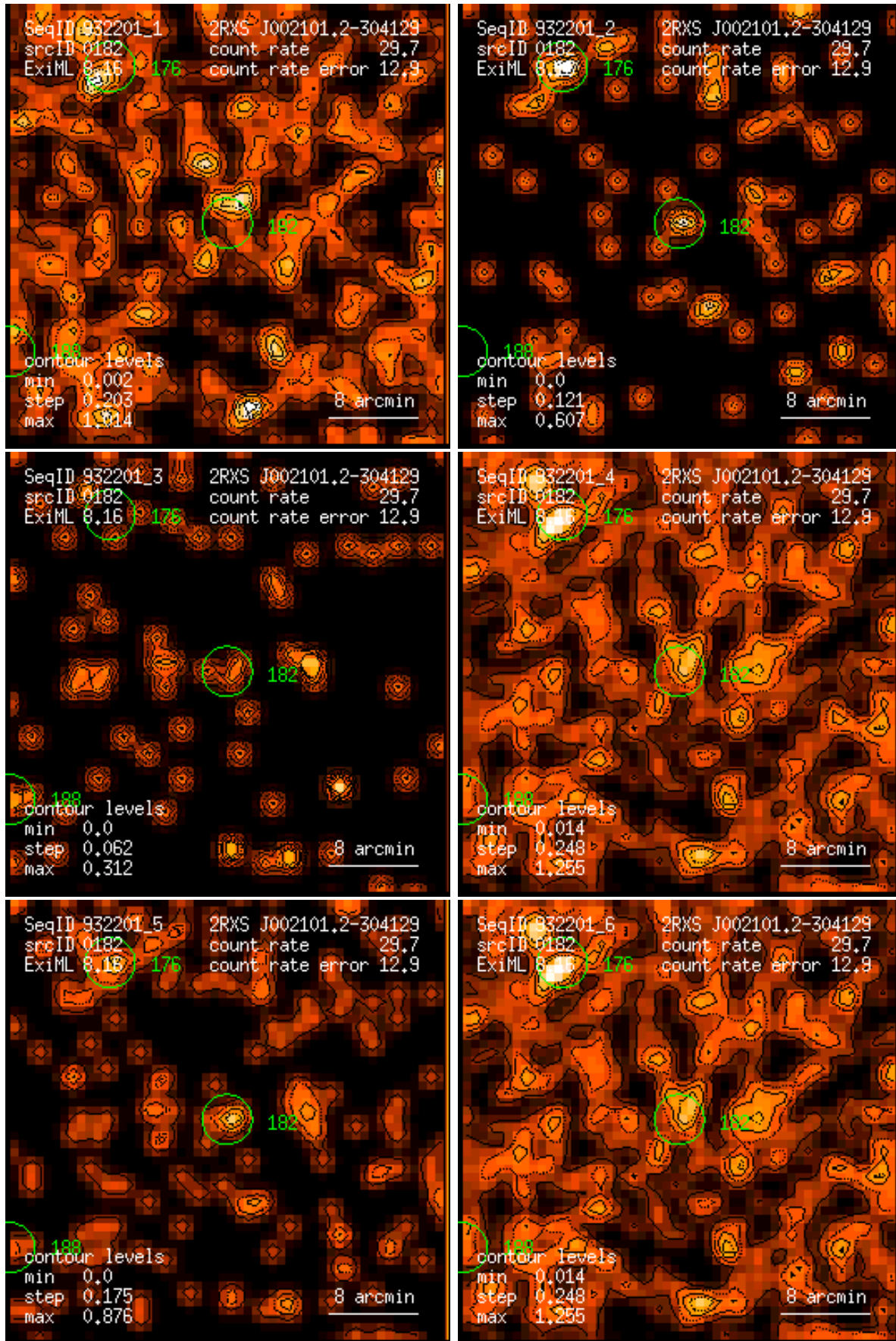
Figure 182: RASS 932201: detection 0182: band rate images, Gaussian filter: (1) PSPC channels 11 – 41, (2) 52 – 90, (3) 91 – 201, (4) 11 – 235, (5) 52 – 201, (6) 11 – 201. Broad band rates in counts/ks. Band rate contour levels in counts/ks/arcmin 2 .
