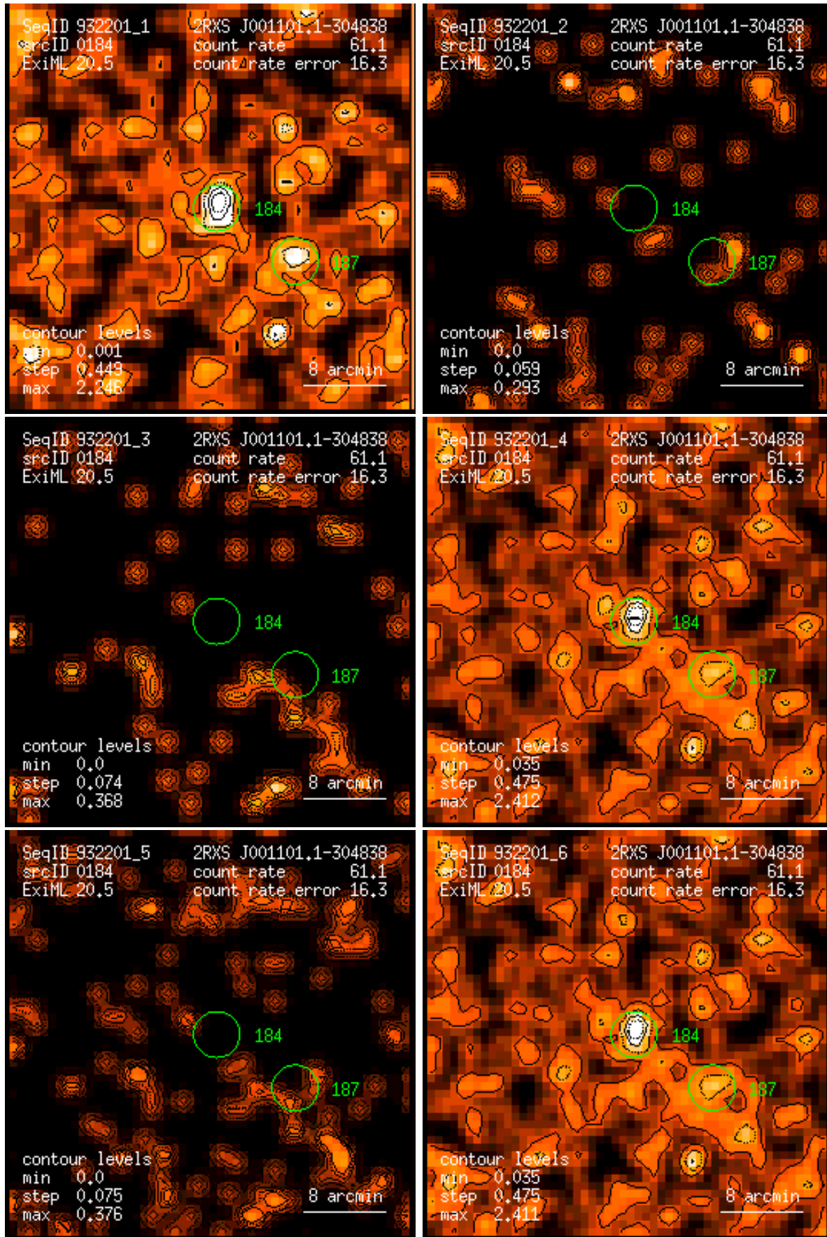
Figure 184: RASS 932201: detection 0184: band rate images, Gaussian filter: (1) PSPC channels 11 – 41, (2) 52 – 90, (3) 91 – 201, (4) 11 – 235, (5) 52 – 201, (6) 11 – 201. Broad band rates in counts/ks. Band rate contour levels in counts/ks/arcmin 2 .
