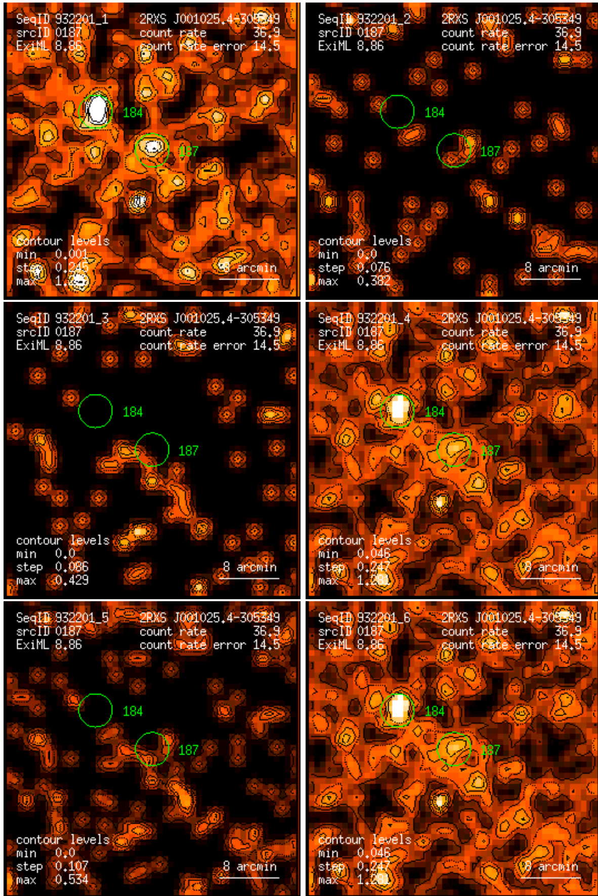
Figure 187: RASS 932201: detection 0187: band rate images, Gaussian filter: (1) PSPC channels 11 – 41, (2) 52 – 90, (3) 91 – 201, (4) 11 – 235, (5) 52 – 201, (6) 11 – 201. Broad band rates in counts/ks. Band rate contour levels in counts/ks/arcmin 2 .
