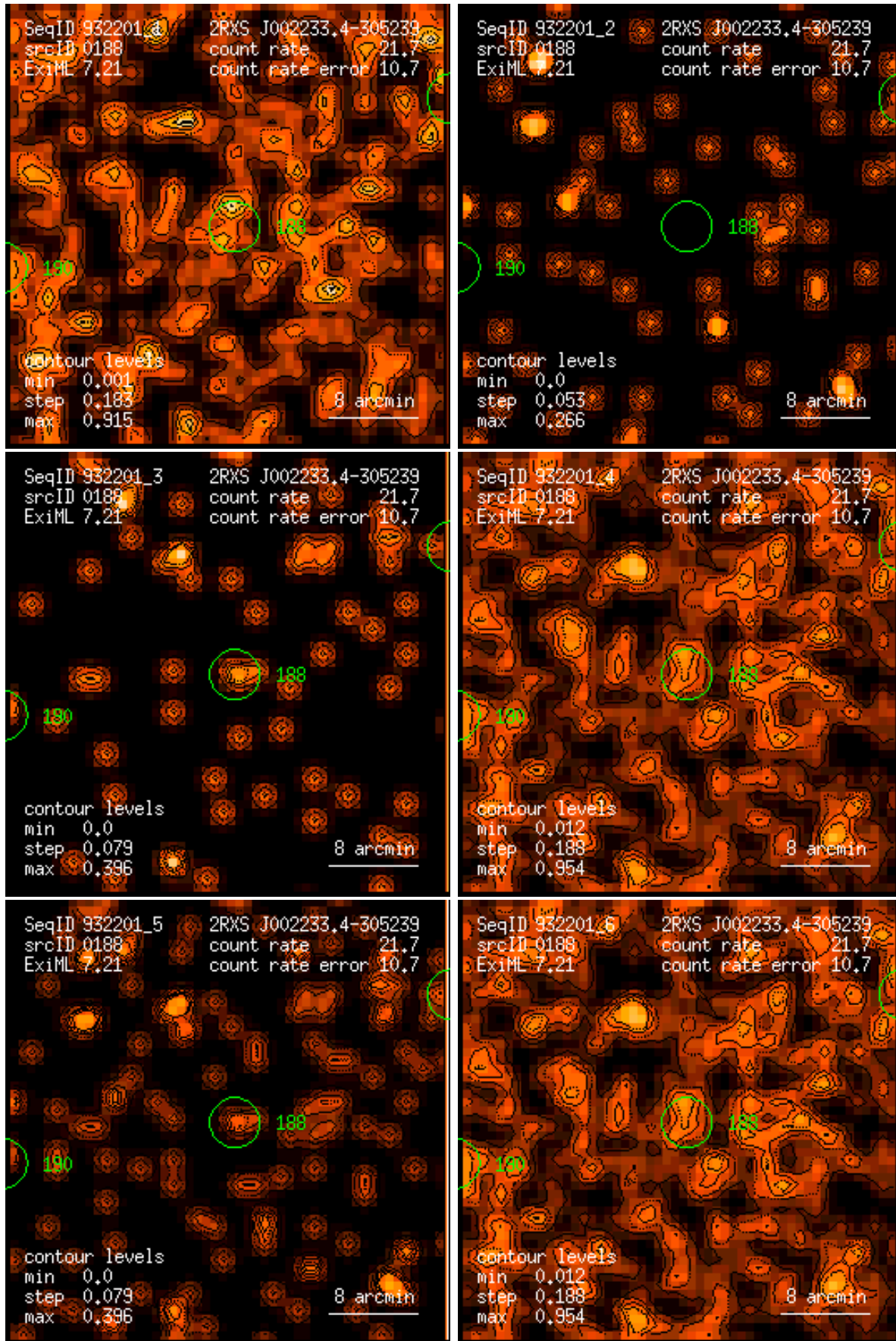
Figure 188: RASS 932201: detection 0188: band rate images, Gaussian filter: (1) PSPC channels 11 – 41, (2) 52 – 90, (3) 91 – 201, (4) 11 – 235, (5) 52 – 201, (6) 11 – 201. Broad band rates in counts/ks. Band rate contour levels in counts/ks/arcmin 2 .
