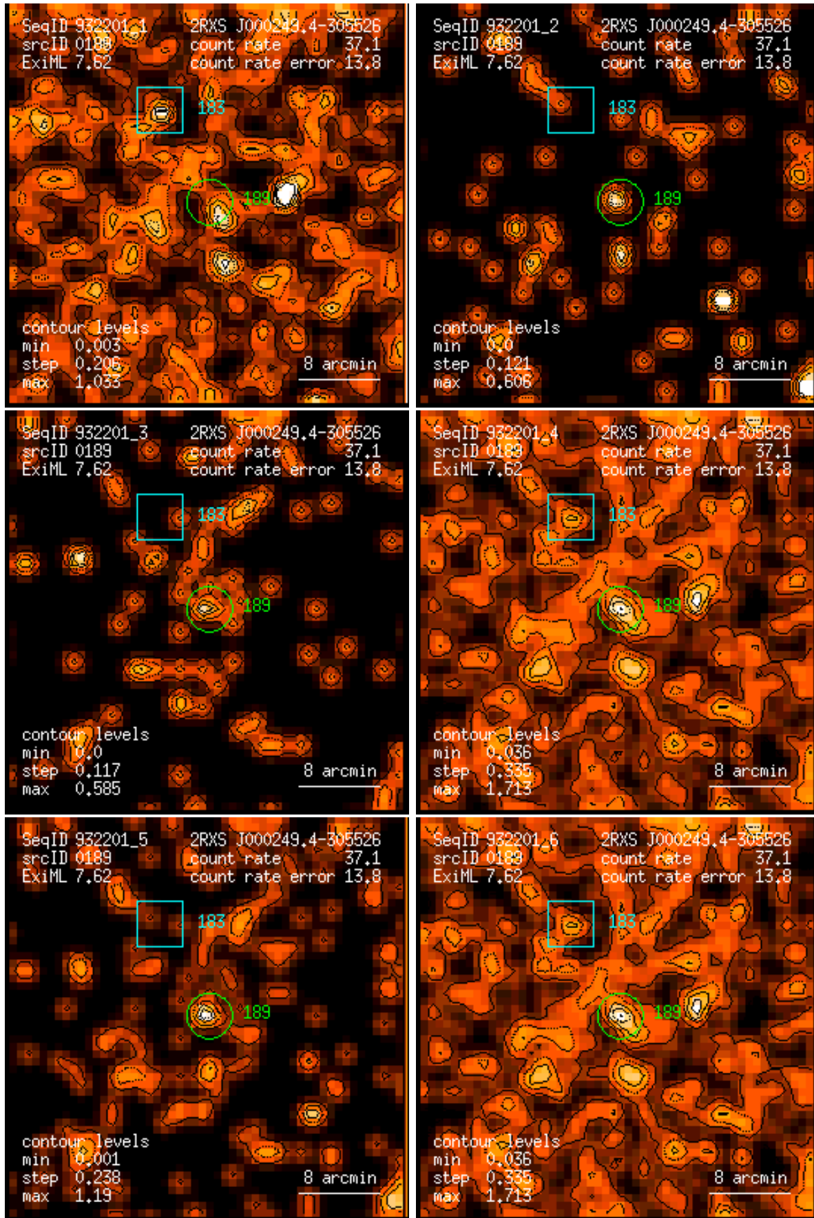
Figure 189: RASS 932201: detection 0189: band rate images, Gaussian filter: (1) PSPC channels 11 – 41, (2) 52 – 90, (3) 91 – 201, (4) 11 – 235, (5) 52 – 201, (6) 11 – 201. Broad band rates in counts/ks. Band rate contour levels in counts/ks/arcmin 2 .
