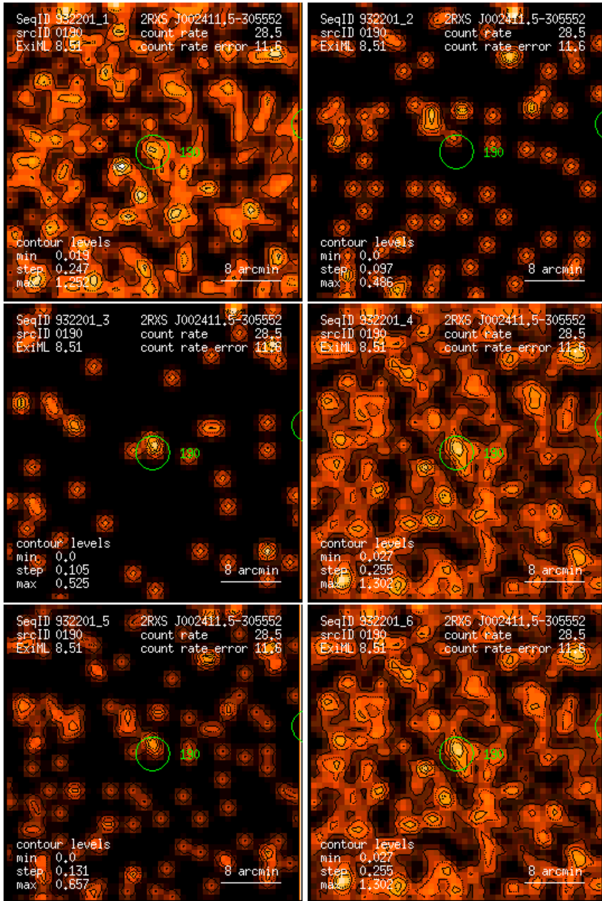
Figure 190: RASS 932201: detection 0190: band rate images, Gaussian filter: (1) PSPC channels 11 – 41, (2) 52 – 90, (3) 91 – 201, (4) 11 – 235, (5) 52 – 201, (6) 11 – 201. Broad band rates in counts/ks. Band rate contour levels in counts/ks/arcmin 2 .
