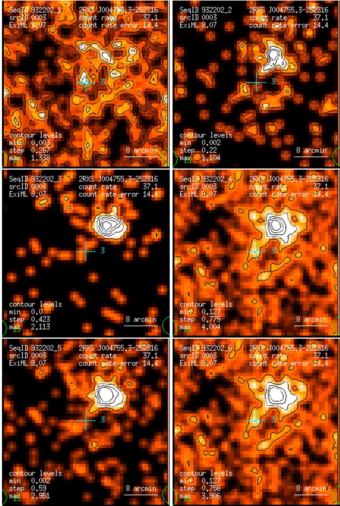
Figure 3: RASS 932202: detection 0003: band rate images, Gaussian filter: (1) PSPC channels 11 – 41, (2) 52 – 90, (3) 91 – 201, (4) 11 – 235, (5) 52 – 201, (6) 11 – 201. Broad band rates in counts/ks. Band rate contour levels in counts/ks/arcmin 2 .
