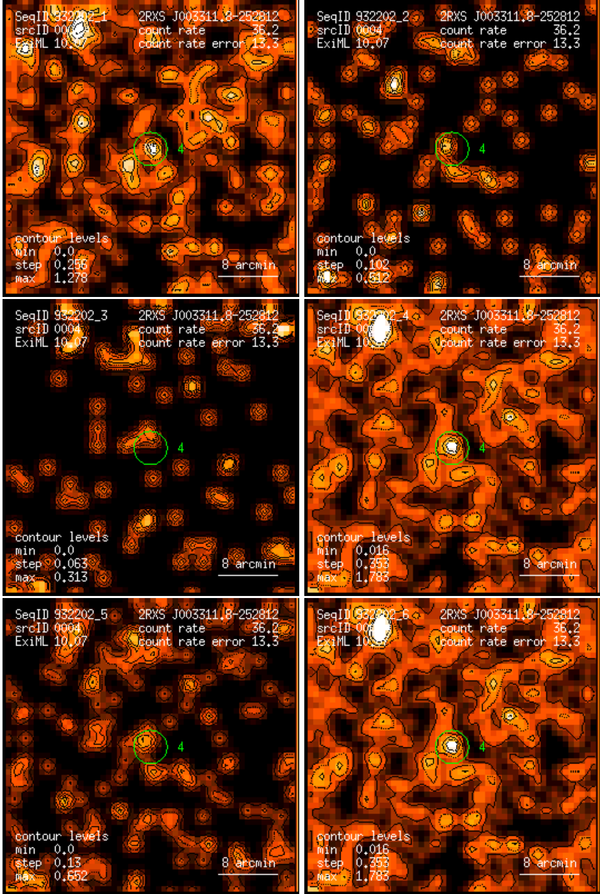
Figure 4: RASS 932202: detection 0004: band rate images, Gaussian filter: (1) PSPC channels 11 – 41, (2) 52 – 90, (3) 91 – 201, (4) 11 – 235, (5) 52 – 201, (6) 11 – 201. Broad band rates in counts/ks. Band rate contour levels in counts/ks/arcmin 2 .
