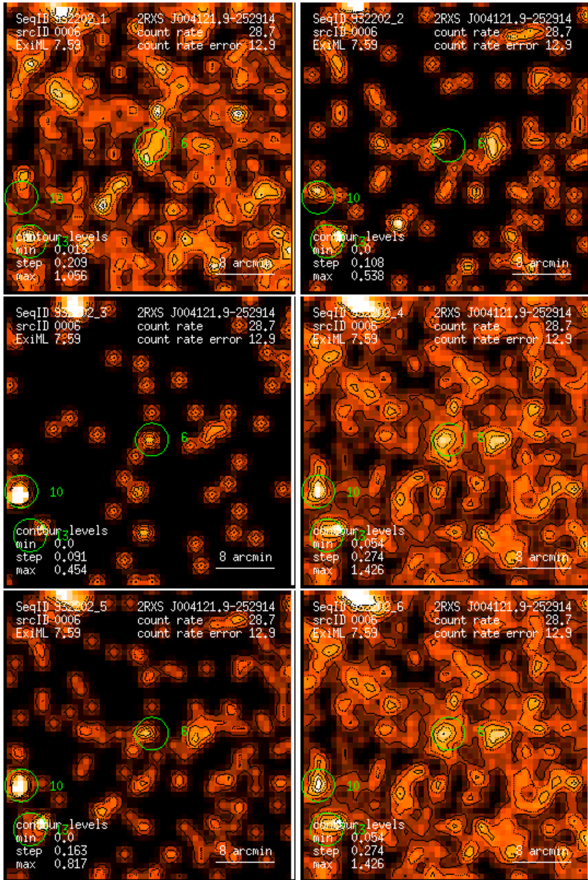
Figure 6: RASS 932202: detection 0006: band rate images, Gaussian filter: (1) PSPC channels 11 – 41, (2) 52 – 90, (3) 91 – 201, (4) 11 – 235, (5) 52 – 201, (6) 11 – 201. Broad band rates in counts/ks. Band rate contour levels in counts/ks/arcmin 2 .
