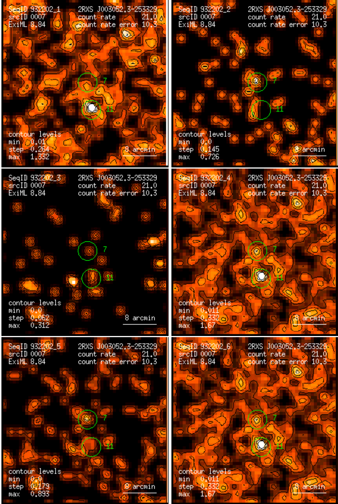
Figure 7: RASS 932202: detection 0007: band rate images, Gaussian filter: (1) PSPC channels 11 – 41, (2) 52 – 90, (3) 91 – 201, (4) 11 – 235, (5) 52 – 201, (6) 11 – 201. Broad band rates in counts/ks. Band rate contour levels in counts/ks/arcmin 2 .
