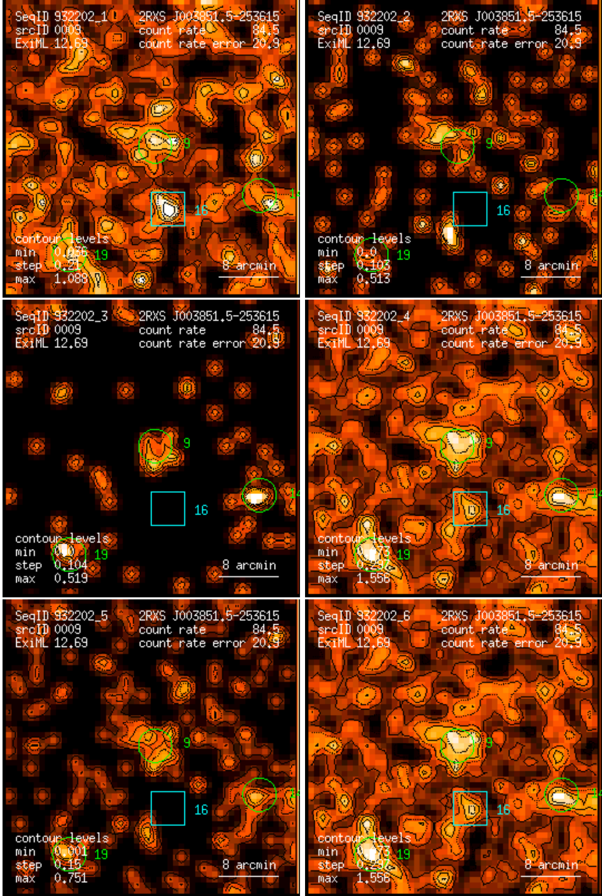
Figure 9: RASS 932202: detection 0009: band rate images, Gaussian filter: (1) PSPC channels 11 – 41, (2) 52 – 90, (3) 91 – 201, (4) 11 – 235, (5) 52 – 201, (6) 11 – 201. Broad band rates in counts/ks. Band rate contour levels in counts/ks/arcmin 2 .
