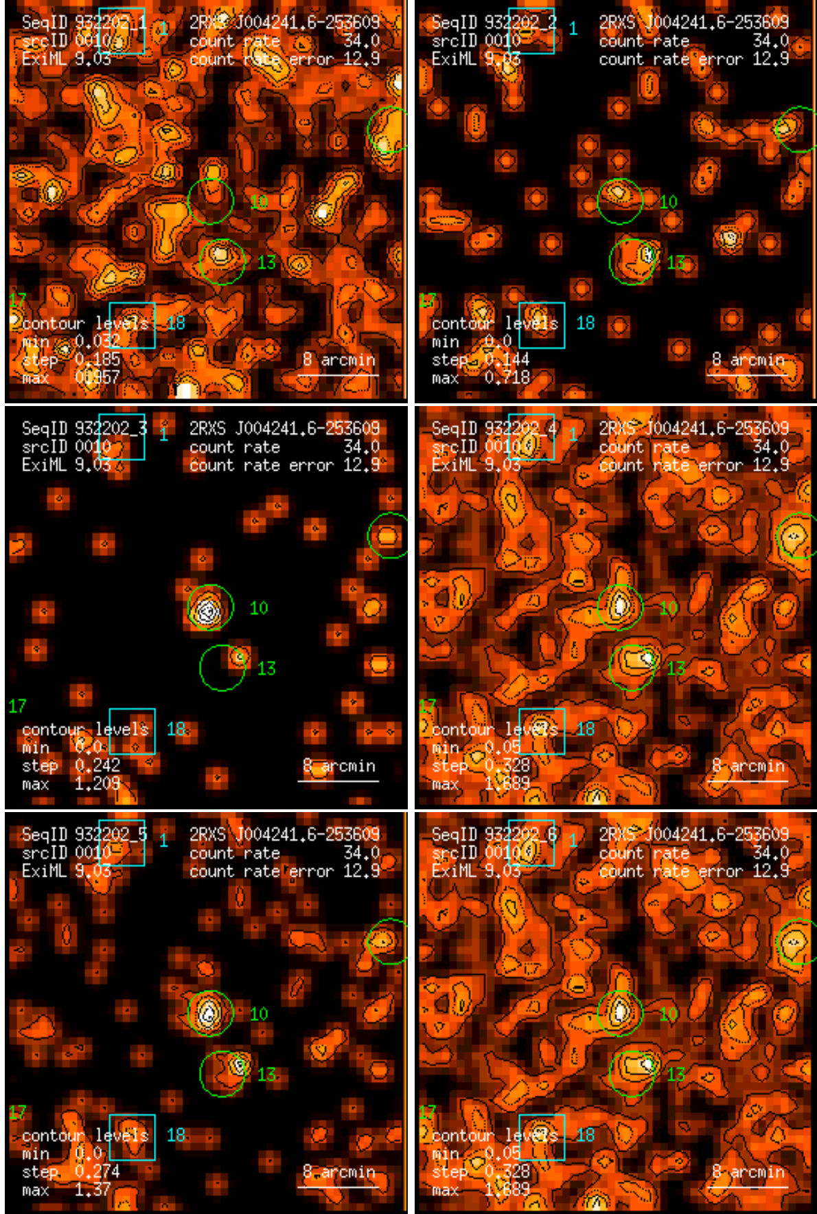
Figure 10: RASS 932202: detection 0010: band rate images, Gaussian filter: (1) PSPC channels 11 – 41, (2) 52 – 90, (3) 91 – 201, (4) 11 – 235, (5) 52 – 201, (6) 11 – 201. Broad band rates in counts/ks. Band rate contour levels in counts/ks/arcmin 2 .
