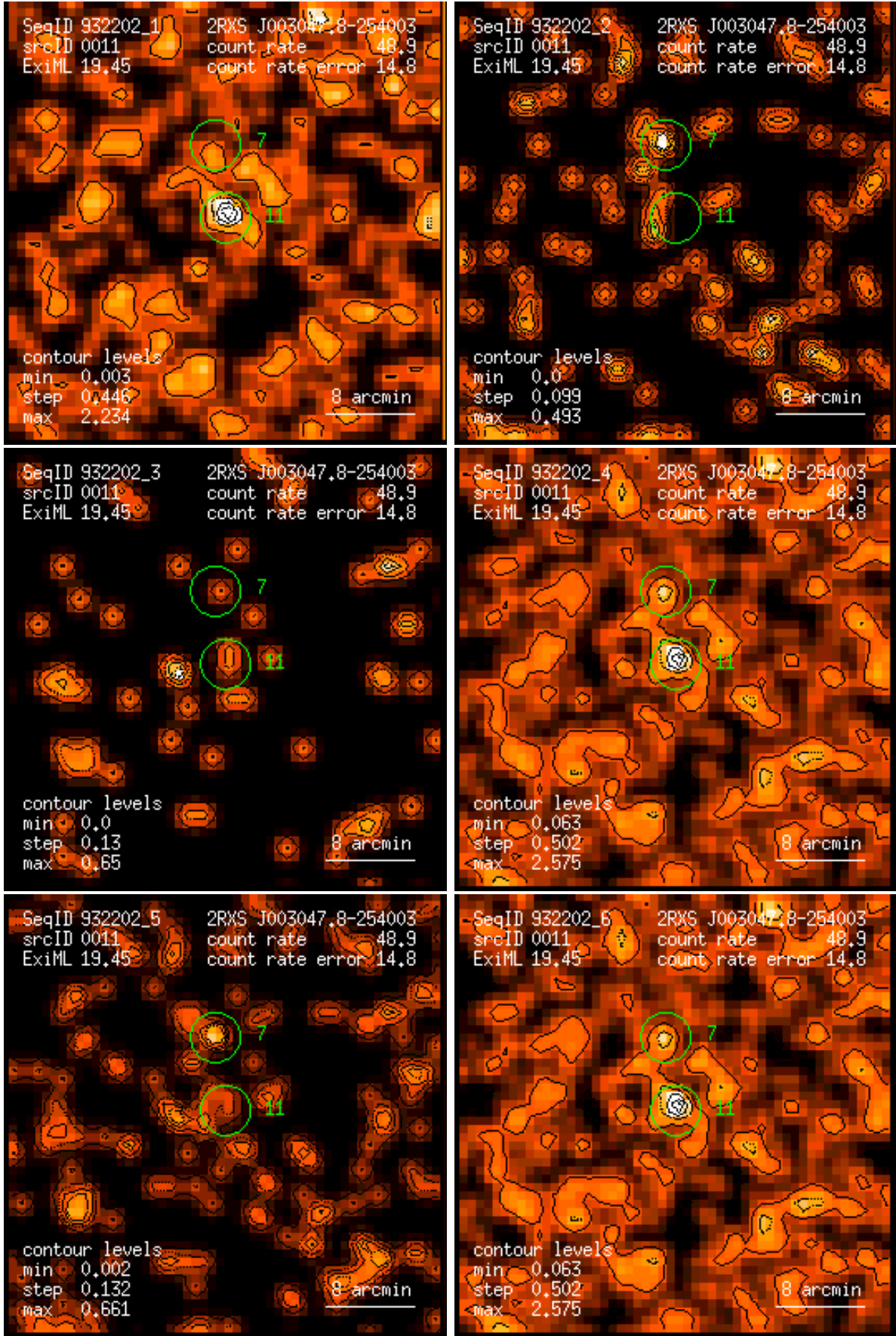
Figure 11: RASS 932202: detection 0011: band rate images, Gaussian filter: (1) PSPC channels 11 – 41, (2) 52 – 90, (3) 91 – 201, (4) 11 – 235, (5) 52 – 201, (6) 11 – 201. Broad band rates in counts/ks. Band rate contour levels in counts/ks/arcmin 2 .
