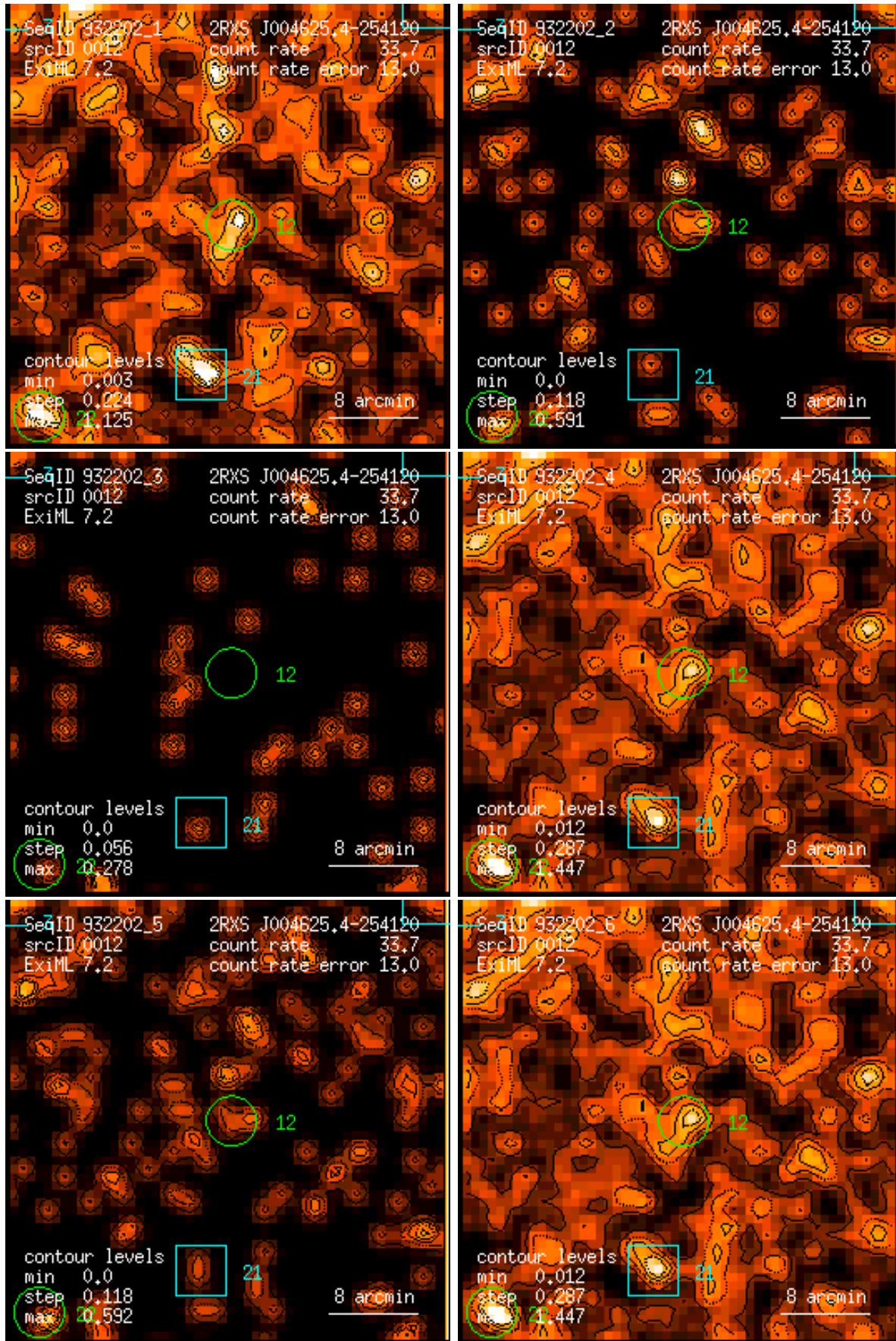
Figure 12: RASS 932202: detection 0012: band rate images, Gaussian filter: (1) PSPC channels 11 – 41, (2) 52 – 90, (3) 91 – 201, (4) 11 – 235, (5) 52 – 201, (6) 11 – 201. Broad band rates in counts/ks. Band rate contour levels in counts/ks/arcmin 2 .
