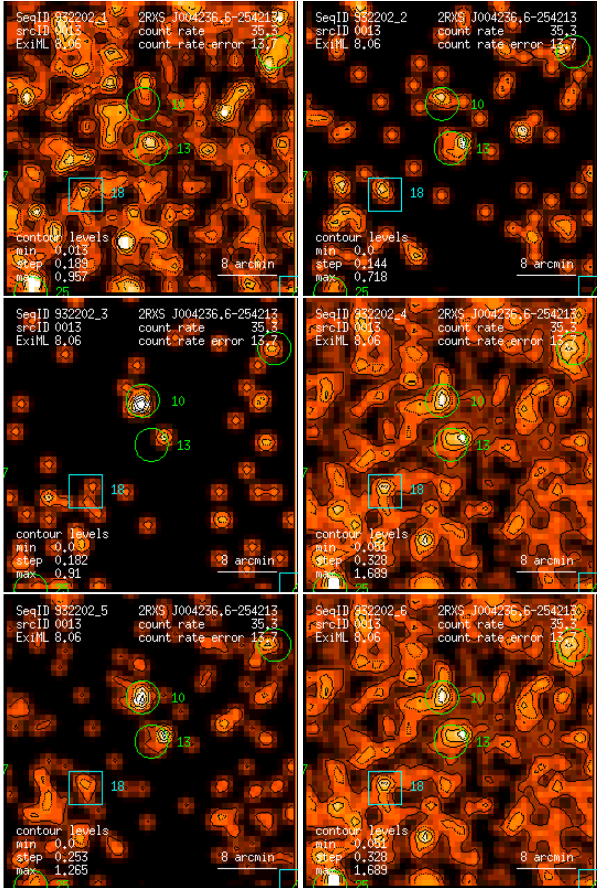
Figure 13: RASS 932202: detection 0013: band rate images, Gaussian filter: (1) PSPC channels 11 – 41, (2) 52 – 90, (3) 91 – 201, (4) 11 – 235, (5) 52 – 201, (6) 11 – 201. Broad band rates in counts/ks. Band rate contour levels in counts/ks/arcmin 2 .
