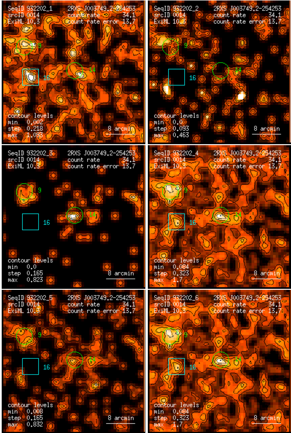
Figure 14: RASS 932202: detection 0014: band rate images, Gaussian filter: (1) PSPC channels 11 – 41, (2) 52 – 90, (3) 91 – 201, (4) 11 – 235, (5) 52 – 201, (6) 11 – 201. Broad band rates in counts/ks. Band rate contour levels in counts/ks/arcmin 2 .
