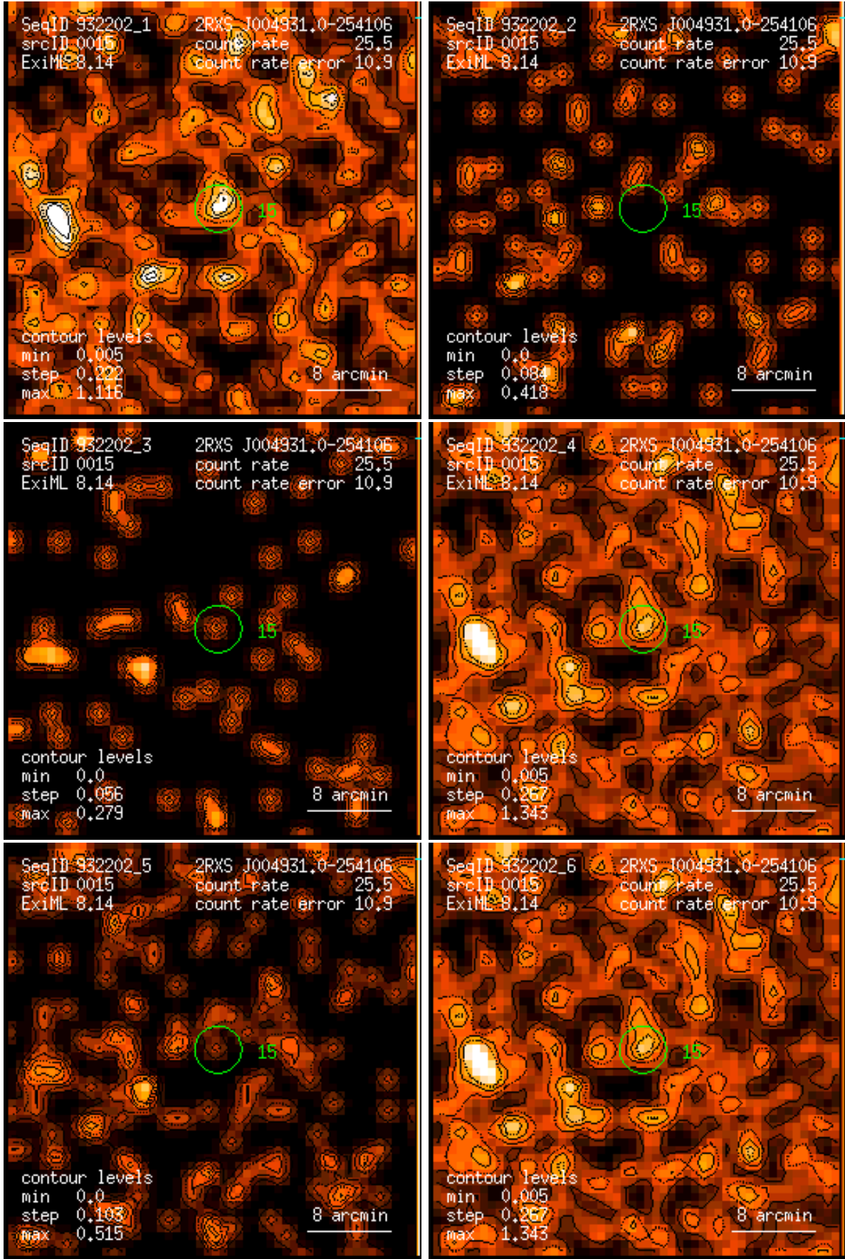
Figure 15: RASS 932202: detection 0015: band rate images, Gaussian filter: (1) PSPC channels 11 – 41, (2) 52 – 90, (3) 91 – 201, (4) 11 – 235, (5) 52 – 201, (6) 11 – 201. Broad band rates in counts/ks. Band rate contour levels in counts/ks/arcmin 2 .
