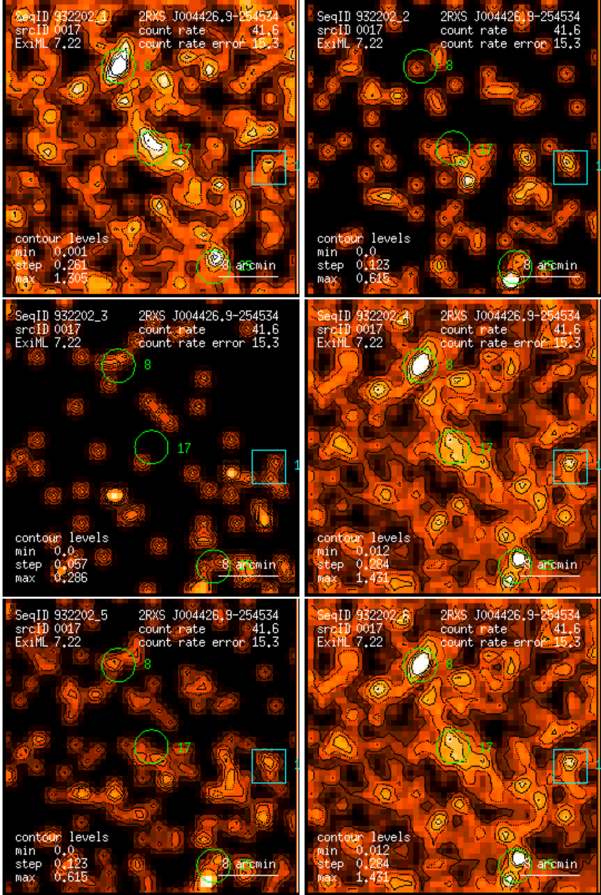
Figure 17: RASS 932202: detection 0017: band rate images, Gaussian filter: (1) PSPC channels 11 – 41, (2) 52 – 90, (3) 91 – 201, (4) 11 – 235, (5) 52 – 201, (6) 11 – 201. Broad band rates in counts/ks. Band rate contour levels in counts/ks/arcmin 2 .
