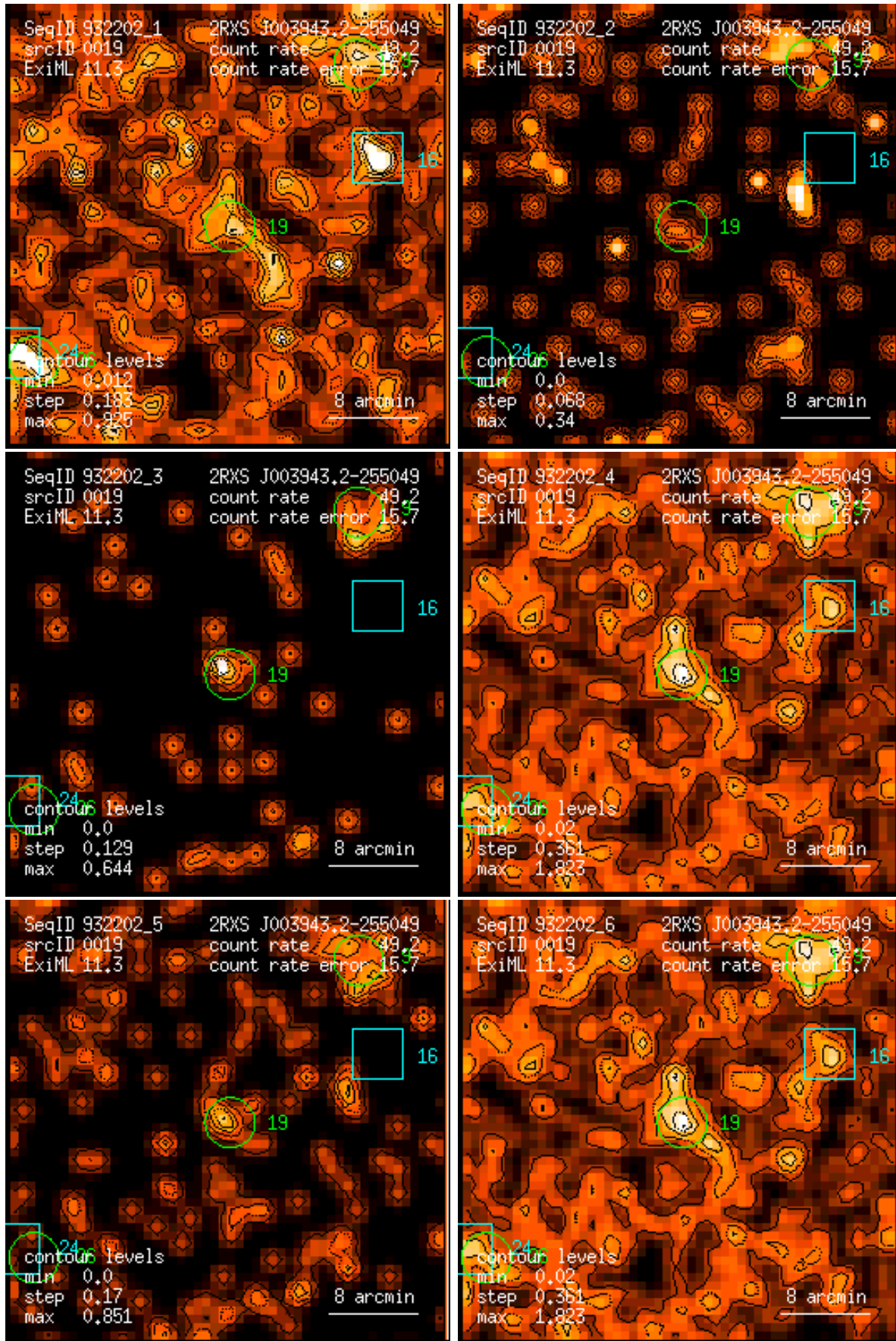
Figure 19: RASS 932202: detection 0019: band rate images, Gaussian filter: (1) PSPC channels 11 – 41, (2) 52 – 90, (3) 91 – 201, (4) 11 – 235, (5) 52 – 201, (6) 11 – 201. Broad band rates in counts/ks. Band rate contour levels in counts/ks/arcmin 2 .
