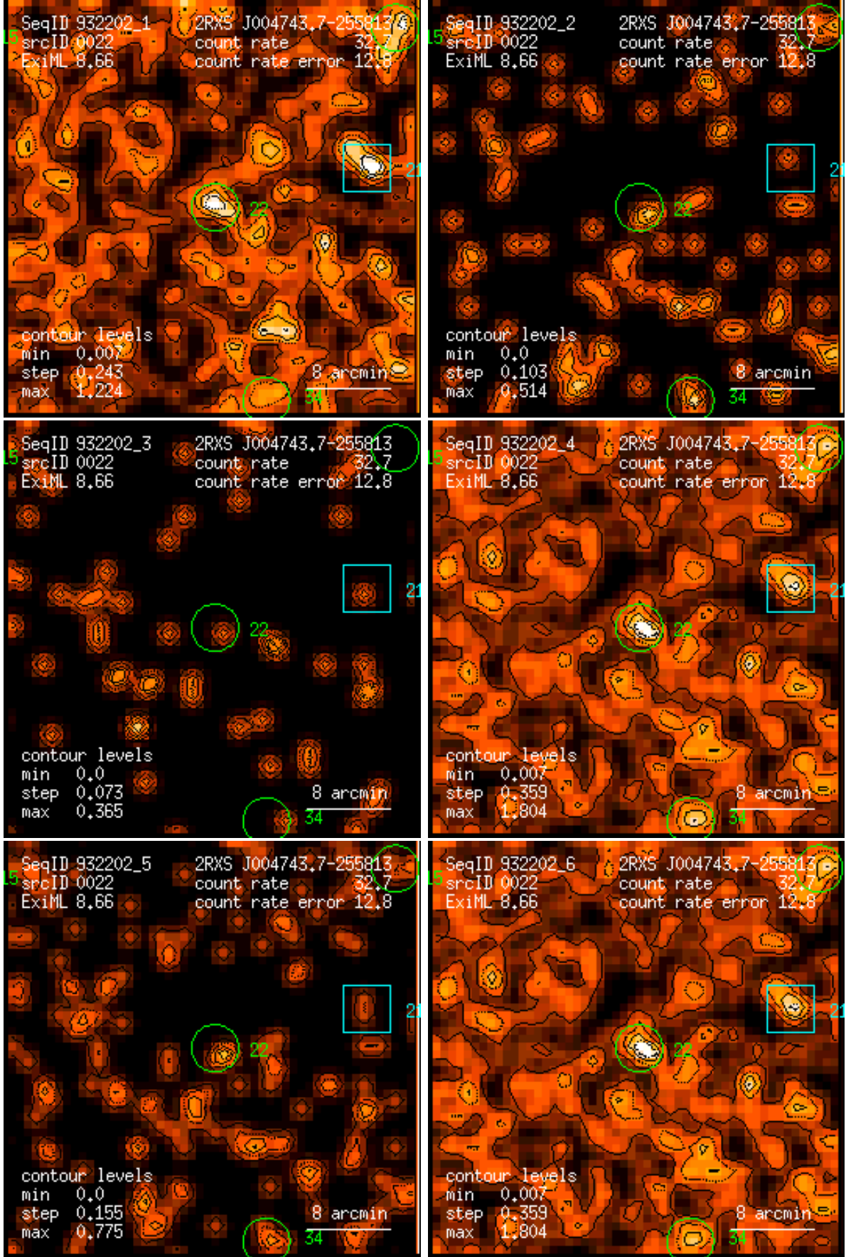
Figure 22: RASS 932202: detection 0022: band rate images, Gaussian filter: (1) PSPC channels 11 – 41, (2) 52 – 90, (3) 91 – 201, (4) 11 – 235, (5) 52 – 201, (6) 11 – 201. Broad band rates in counts/ks. Band rate contour levels in counts/ks/arcmin 2 .
