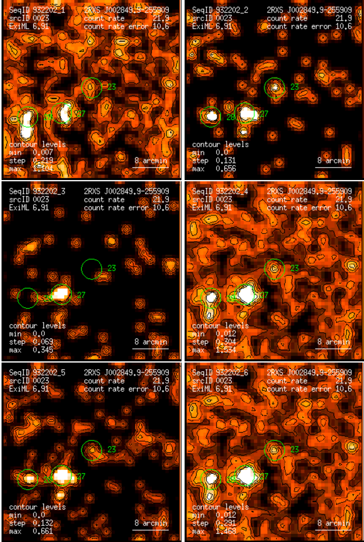
Figure 23: RASS 932202: detection 0023: band rate images, Gaussian filter: (1) PSPC channels 11 – 41, (2) 52 – 90, (3) 91 – 201, (4) 11 – 235, (5) 52 – 201, (6) 11 – 201. Broad band rates in counts/ks. Band rate contour levels in counts/ks/arcmin 2 .
