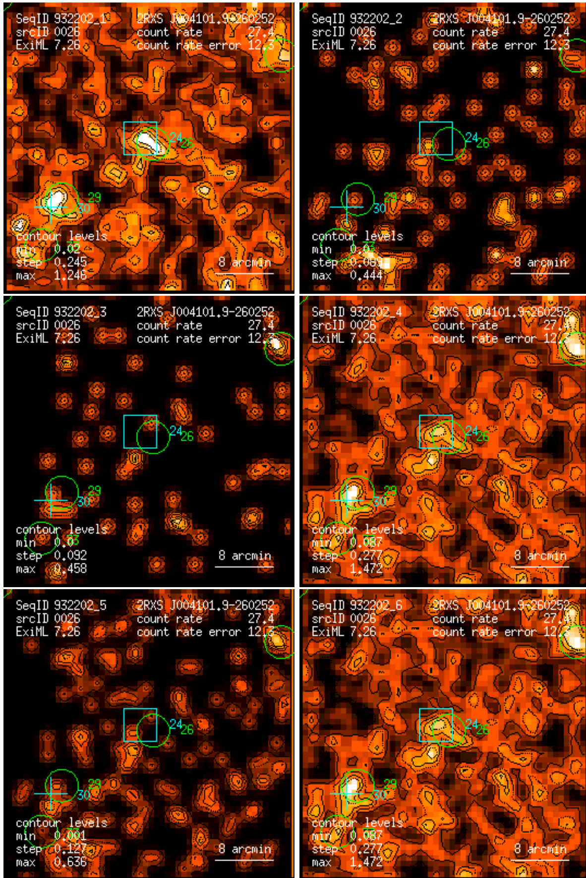
Figure 26: RASS 932202: detection 0026: band rate images, Gaussian filter: (1) PSPC channels 11 – 41, (2) 52 – 90, (3) 91 – 201, (4) 11 – 235, (5) 52 – 201, (6) 11 – 201. Broad band rates in counts/ks. Band rate contour levels in counts/ks/arcmin 2 .
