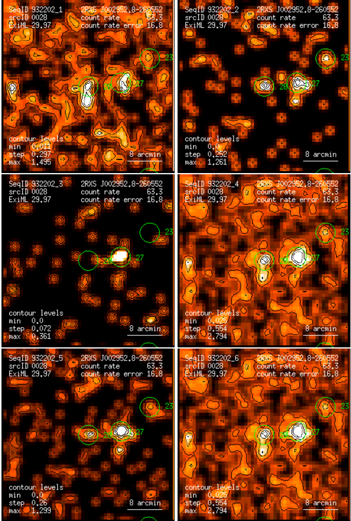
Figure 28: RASS 932202: detection 0028: band rate images, Gaussian filter: (1) PSPC channels 11 – 41, (2) 52 – 90, (3) 91 – 201, (4) 11 – 235, (5) 52 – 201, (6) 11 – 201. Broad band rates in counts/ks. Band rate contour levels in counts/ks/arcmin 2 .
