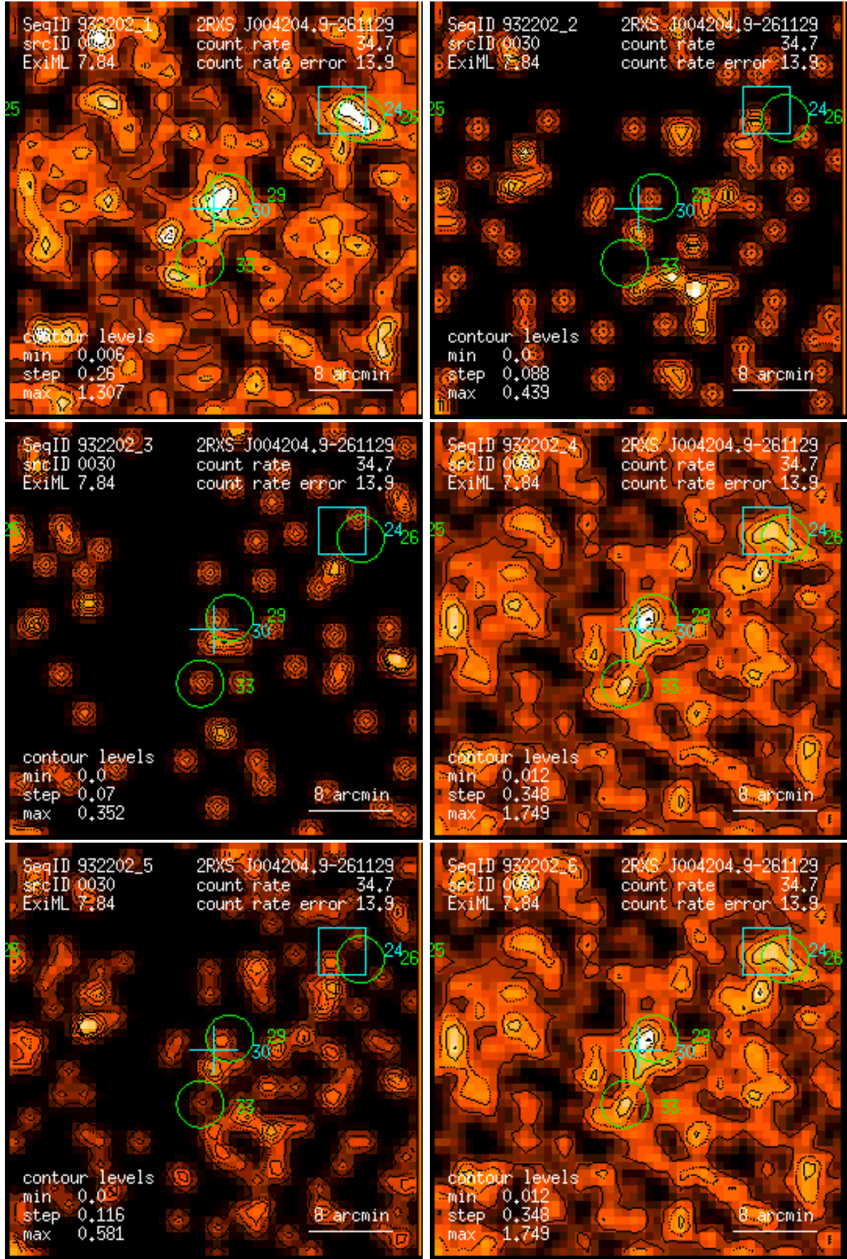
Figure 30: RASS 932202: detection 0030: band rate images, Gaussian filter: (1) PSPC channels 11 – 41, (2) 52 – 90, (3) 91 – 201, (4) 11 – 235, (5) 52 – 201, (6) 11 – 201. Broad band rates in counts/ks. Band rate contour levels in counts/ks/arcmin 2 .
