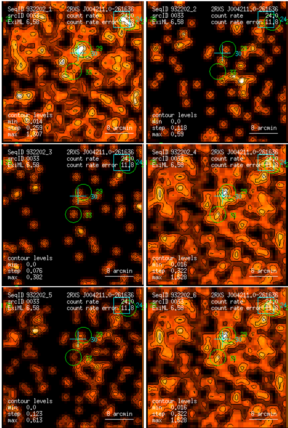
Figure 33: RASS 932202: detection 0033: band rate images, Gaussian filter: (1) PSPC channels 11 – 41, (2) 52 – 90, (3) 91 – 201, (4) 11 – 235, (5) 52 – 201, (6) 11 – 201. Broad band rates in counts/ks. Band rate contour levels in counts/ks/arcmin 2 .
