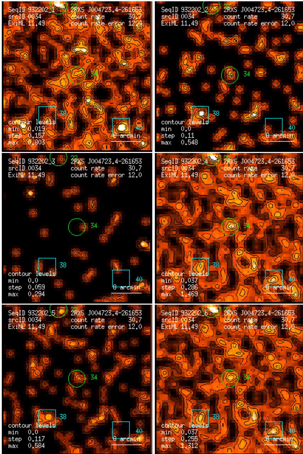
Figure 34: RASS 932202: detection 0034: band rate images, Gaussian filter: (1) PSPC channels 11 – 41, (2) 52 – 90, (3) 91 – 201, (4) 11 – 235, (5) 52 – 201, (6) 11 – 201. Broad band rates in counts/ks. Band rate contour levels in counts/ks/arcmin 2 .
