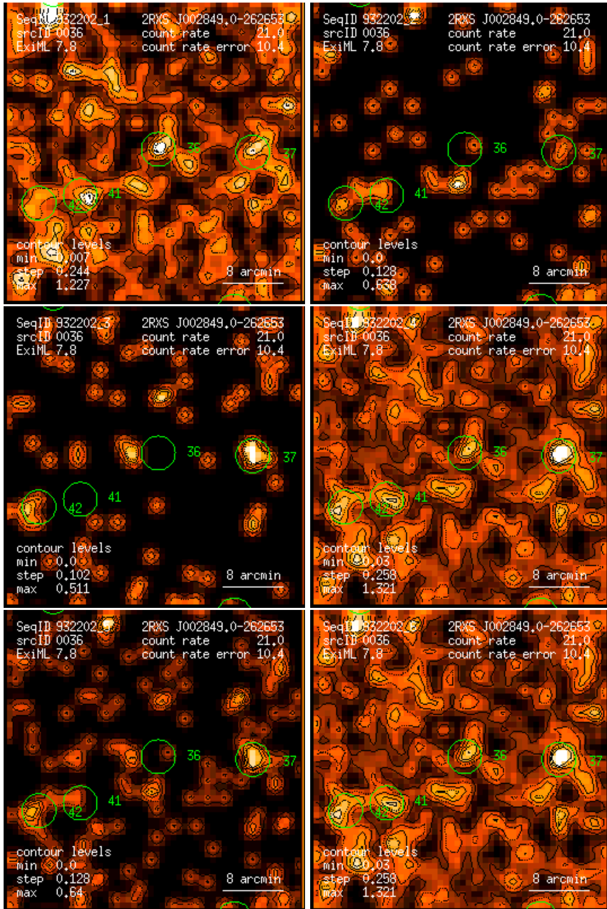
Figure 36: RASS 932202: detection 0036: band rate images, Gaussian filter: (1) PSPC channels 11 – 41, (2) 52 – 90, (3) 91 – 201, (4) 11 – 235, (5) 52 – 201, (6) 11 – 201. Broad band rates in counts/ks. Band rate contour levels in counts/ks/arcmin 2 .
