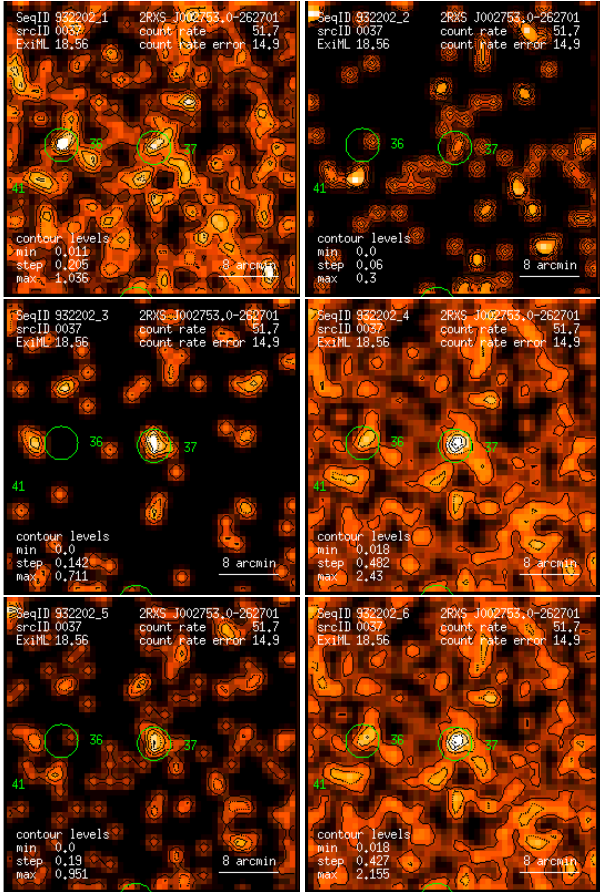
Figure 37: RASS 932202: detection 0037: band rate images, Gaussian filter: (1) PSPC channels 11 – 41, (2) 52 – 90, (3) 91 – 201, (4) 11 – 235, (5) 52 – 201, (6) 11 – 201. Broad band rates in counts/ks. Band rate contour levels in counts/ks/arcmin 2 .
