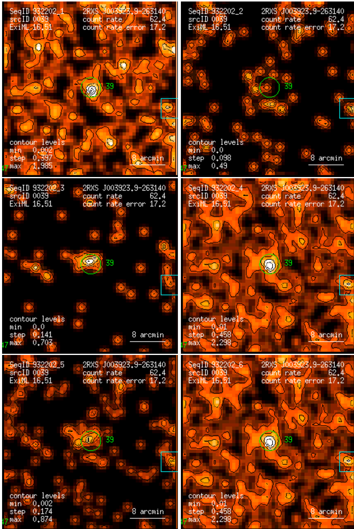
Figure 39: RASS 932202: detection 0039: band rate images, Gaussian filter: (1) PSPC channels 11 – 41, (2) 52 – 90, (3) 91 – 201, (4) 11 – 235, (5) 52 – 201, (6) 11 – 201. Broad band rates in counts/ks. Band rate contour levels in counts/ks/arcmin 2 .
