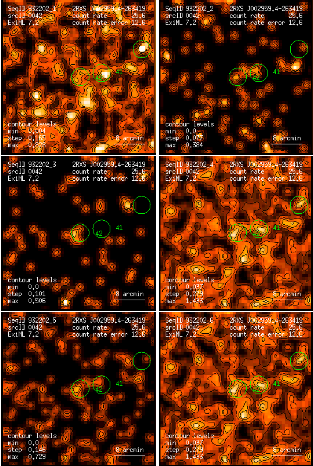
Figure 42: RASS 932202: detection 0042: band rate images, Gaussian filter: (1) PSPC channels 11 – 41, (2) 52 – 90, (3) 91 – 201, (4) 11 – 235, (5) 52 – 201, (6) 11 – 201. Broad band rates in counts/ks. Band rate contour levels in counts/ks/arcmin 2 .
